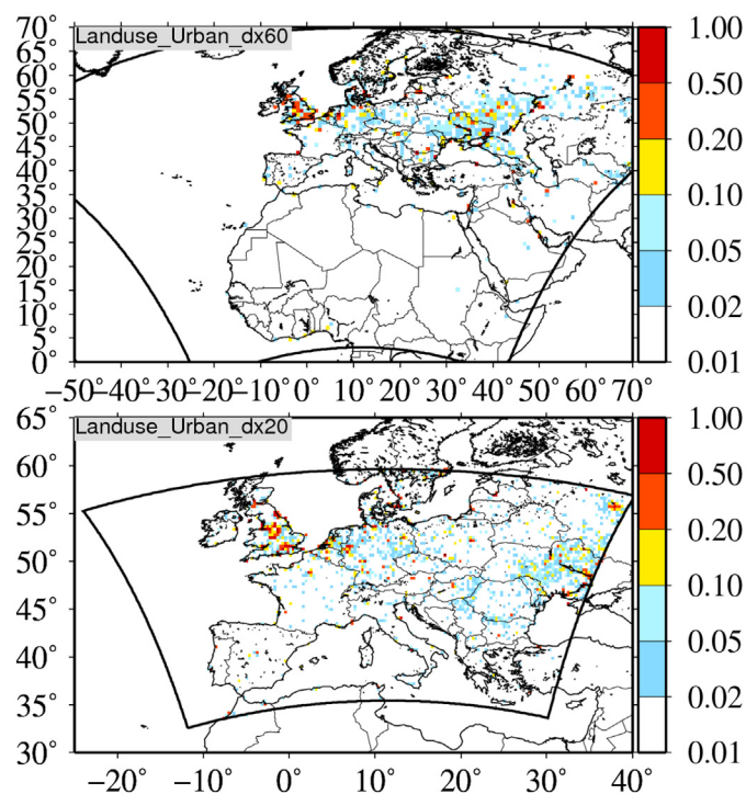
Fig. 1. The two simulation domains used in this study. Colors indicate the percentage of 'urban' landuse in the grid cell.
