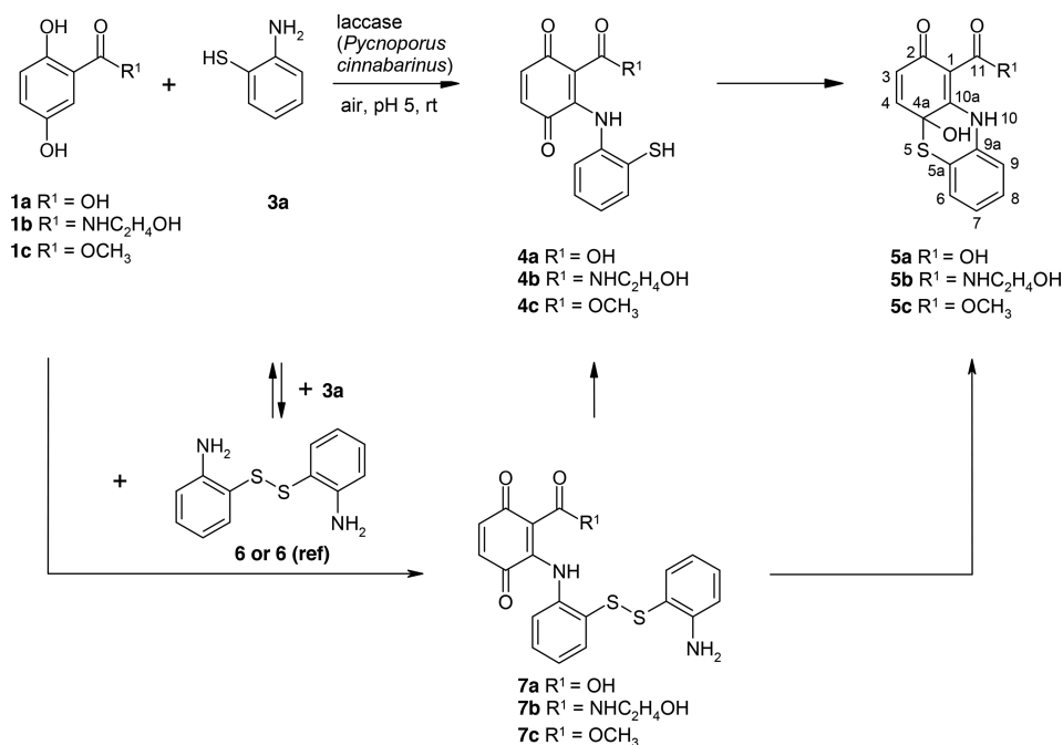
Scheme 5. Laccase-Catalyzed Reactions of 2,5-Dihydroxybenzoic Acid Derivatives 1a–1c with 2-Aminothiophenol 3a, with Its Dimer 6 or with the Commercially Available Reference 2-Aminophenyl Disulfide (6(ref)) for the Synthesis of Adducts 4a–4c and 7a–7c and the Cyclization Products 4a-Hydroxy-2-oxo-phenothiazines 5a–5c Using 0.5 U Laccase of P. cinnabarinus as the Catalyst in Sodium Acetate Buffer (pH 5; Reactant Concentration, 1 mM)
