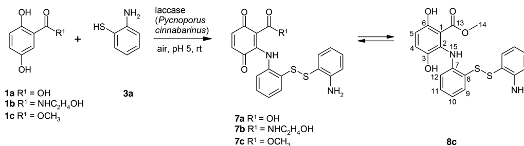
Scheme 4. Laccase-Catalyzed Reaction of 2,5-Dihydroxybenzoic Acid Derivatives 1a–1c with 2-Aminothiophenol 3a for the Synthesis of Adducts 7a–7c and 8c Using 0.5 U Laccase of P. cinnabarinus as the Catalyst in Sodium Acetate Buffer (pH 5; Reactant Concentration, 1 mM)
