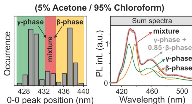
Figure 4. Histogram of the 0-0 peak positions of 210 aggregates assembled with 5% acetone and 95% chloroform vapor ratios. Two populations corresponding to the \beta -phase (orange) and the \gamma -phase (green) can be distinguished. On the right a sum spectrum is shown for the aggregates marked by red in the histogram. This spectrum is described by a superposition (grey) of \beta -phase (orange) and \gamma -phase (green) spectra. In these aggregates both phases are clearly present.
