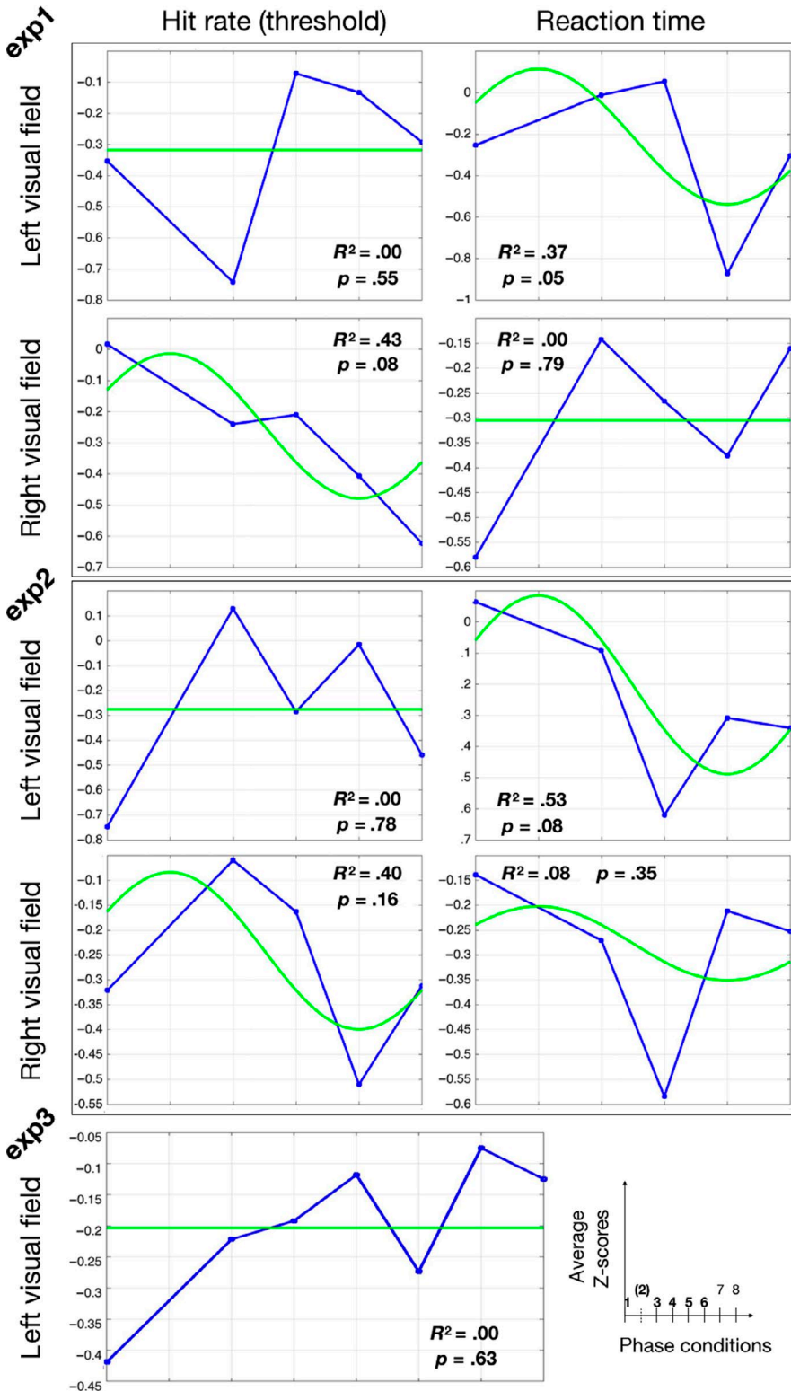
FIGURE 2 Phase-aligned group average results. Individual observed results (contrast thresholds and mean RT in exp 1, accuracy and mean RT in exp 2, hit rate in exp 3) were Z-scored, then phase-shifted such that the absolute peak value was in phase slot “2” for each participant, then averaged across participants (blue lines). The group data point for phase slot “2” was left out of graphs and analysis, as it was an average of the individual datapoints used for phase alignment. tACS-phase modulation of behavioral measures should result in a one-cycle sinusoidal pattern over the remaining phase conditions, with its peak at phase slot 2. Thus phase-locked best fitting sinusoids are shown in green. Above each graph, we present the goodness of fit of these sinusoidal fits, expressed by R-squared (Rsq), and the p -value to come out of a permutation test of the associated relevance value (a measure reflecting both the variance explained and the extent of modulation, see Methods) [Colour figure can be viewed at wileyonlinelibrary.com ]
