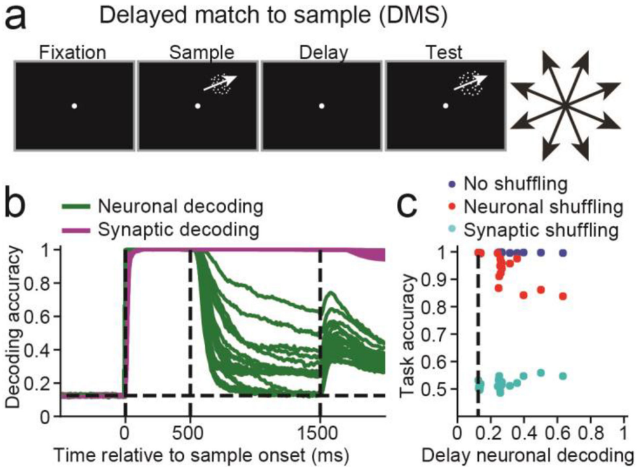
Figure 2. Delayed match-to-sample (DMS) task.
