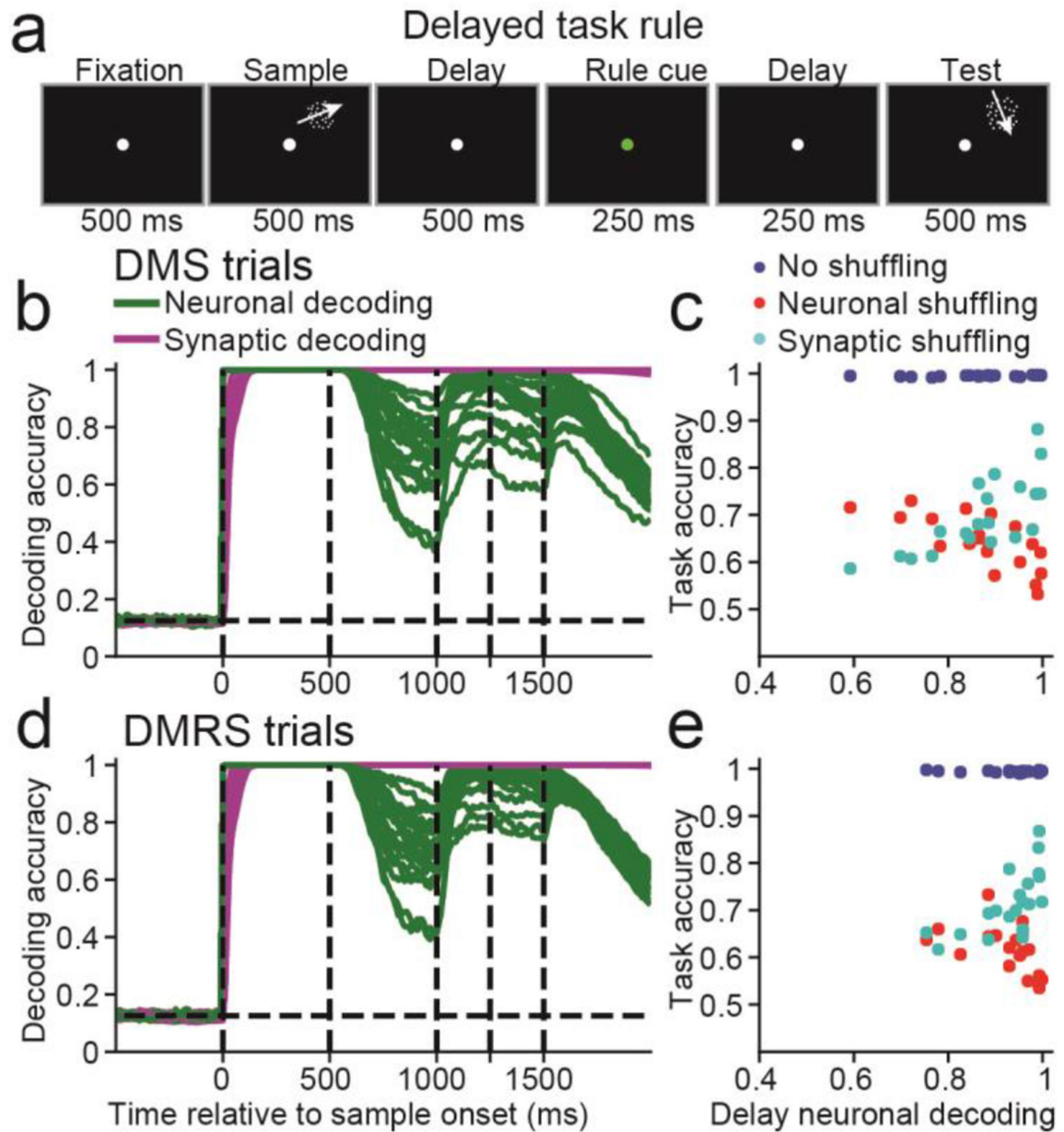
Figure 4. Delayed cue task.
