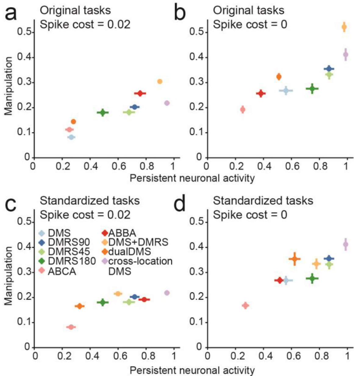
Figure 7. The relationship between manipulation and stimulus-selective persistent activity.
