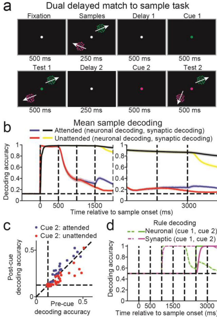
Figure 6. Dual delayed match-to-sample task.
