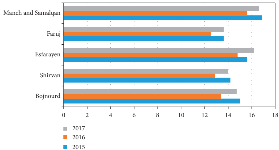
FIGURE 2: Average annual temperature (°C) in North Khorasan cities, Iran, from 2015 to 2017.
