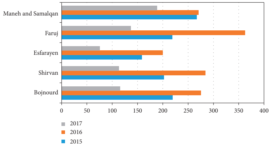
FIGURE 1: Average annual rainfall (mm) in North Khorasan cities, Iran, from 2015 to 2017.
