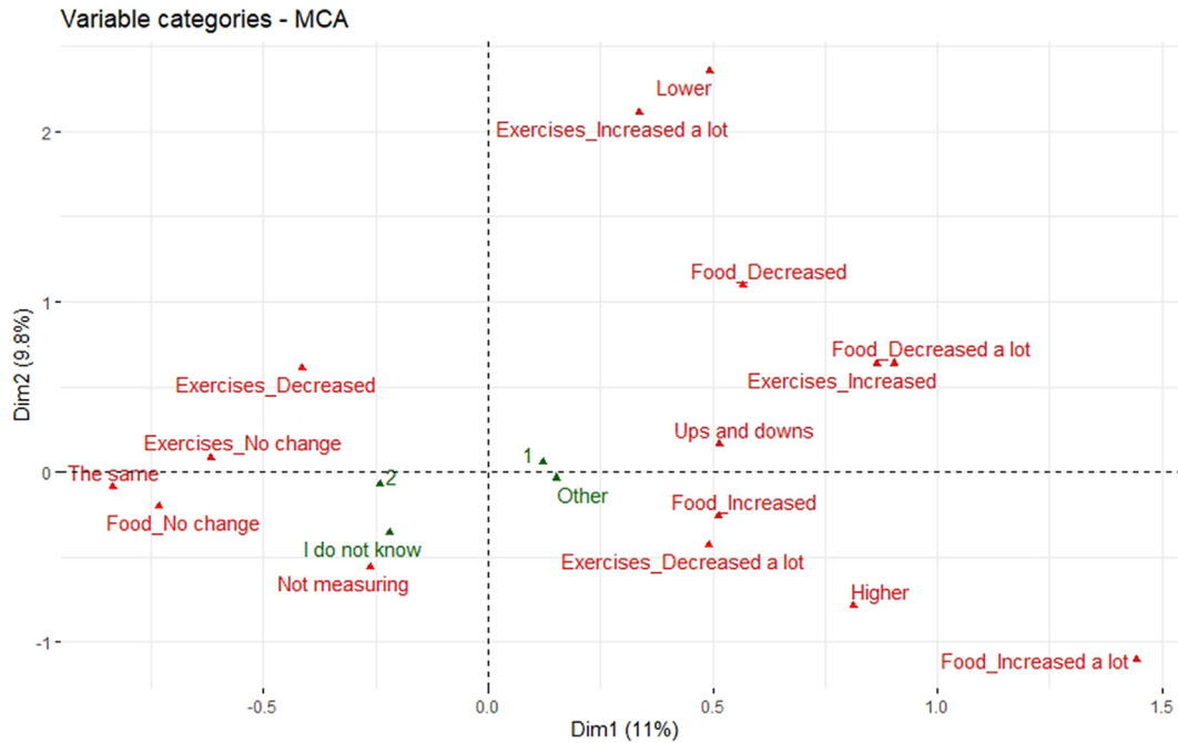
Fig. 2 – MCA for glycemya, food consumption, physical activities, and type of diabetes (supplementary).
