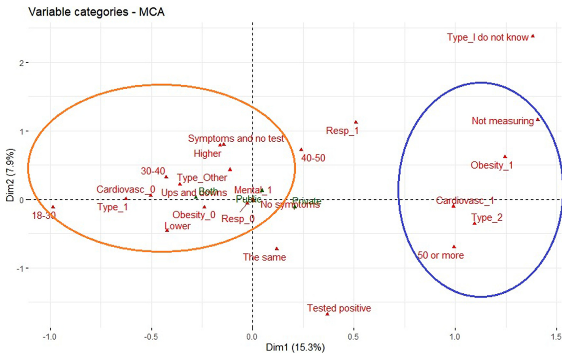
Fig. 1 – MCA for prevalence of cardiovascular diseases, obesity, mental disorders, respiratory diseases, type of diabetes, age (the horizontal axis is a progression of ages of the respondents), symptoms of COVID-19, health system, symptoms (supplementary), and glycaemic measurements (supplementary).
