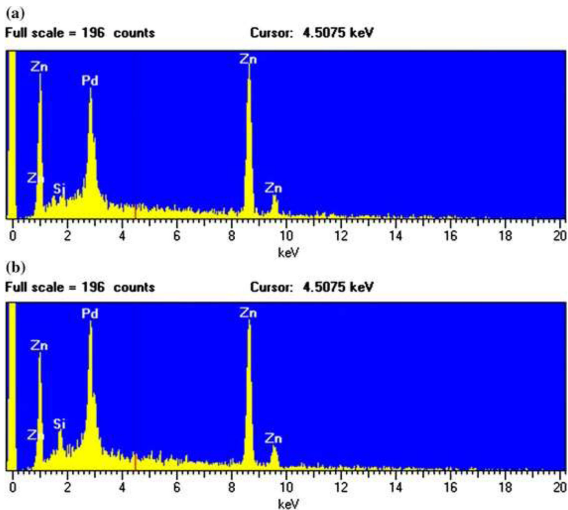
Figure 1. EDS images of the industrial-derived (a) and consumer products-derived nano-ZnO (b)
