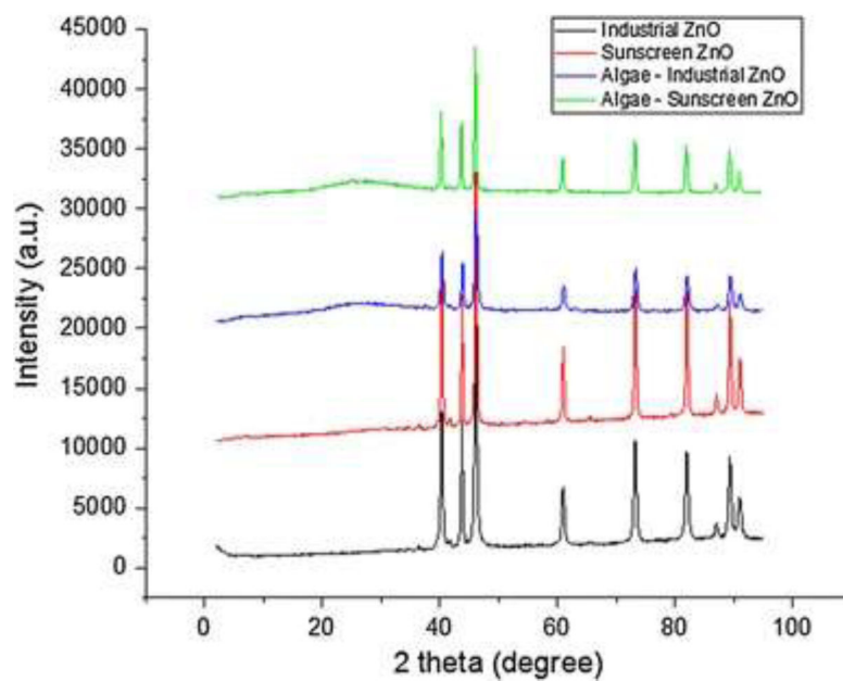
Figure 4. X-ray diffractograms (Fe K \alpha radiation, \lambda = 1.9373 \text{ \AA} ) of industrial nano-ZnO (nZnO, black), sunscreen nZnO (red), algae-industrial nZnO (blue), and algae-sunscreen nZnO (green)
