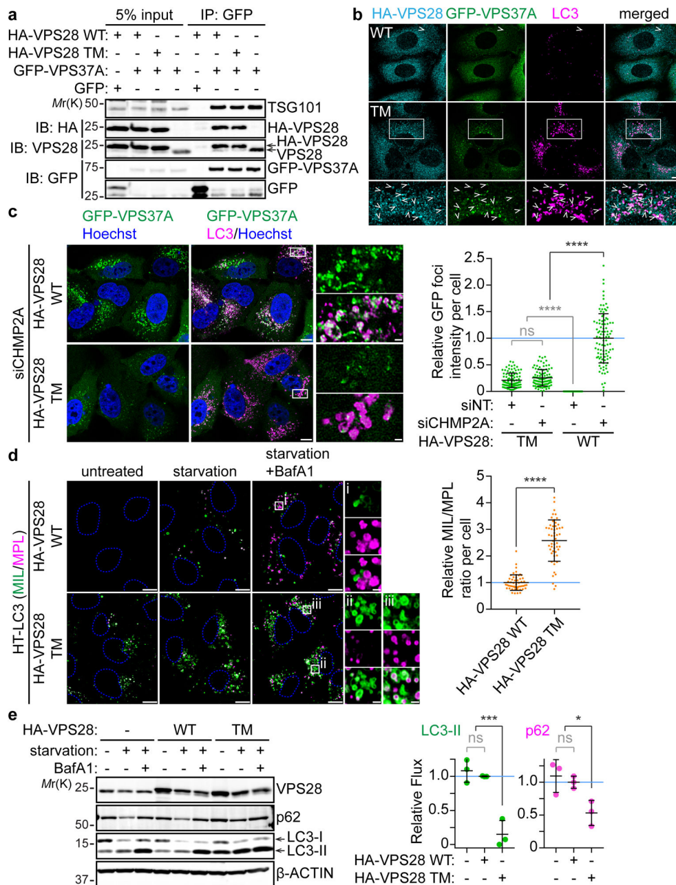
Fig. 4: Helical contacts are required for phagophore closure in autophagy VPS37A -knockout ( a-c ) and wild-type ( d,e ) U-2 OS cells stably expressing GFP- VPS37A and HaloTag(HT)-LC3, respectively, were transduced with lentiviruses encoding HA- VPS28 WT or HA- VPS28 TM for 4 days. a , Western blot analysis of whole-cell lysates (input) and immunoprecipitates (IP) from the indicated cells. b,c , Confocal images of cells that were starved for 3h and stained for HA and LC3 ( b ) or nucleofected with non-targeting siRNA (siNT) or CHMP2A siRNA (siCHMP2A) for 48 h and stained for LC3 and Hoechst 33342 ( c ). Arrowheads in b indicate colocalization of HA-tagged VPS28 (WT or T-2) with GFP- VPS37A on LC3-positive structures. In c , the fluorescence intensity of GFP- VPS37A foci normalized to total GFP intensity per cell is shown relative to the mean of the control HA-
