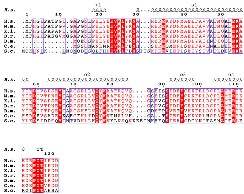
Extended Data Fig. 2. Sequence alignment of VPS28 orthologs Secondary structure displayed above the alignment is derived from the human ESCRT-I head structure. Alignment was generated using ClustalW and ESPrift.
