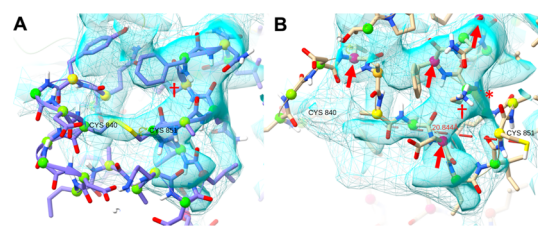
Figure 5. In chain A of PDB: 6VSB, the density strongly suggests \alpha -helix spanning residues 849–856 and a disulfide bond between Cys840 and Cys851. (A) As modeled in this study, colored balls on CA atoms are ISOLDE markup indicating Ramachandran status (green = favored; hot pink = outlier). Lysine 854 (dagger) is pointing into the page, where it forms a salt bridge with Asp614 of an adjacent chain. (B) Starting chain A model of DESRES-ANTON-11021571 has Cys840 and Cys851 about 20 Å apart. There are four severe Ramachandran outliers (red arrows) and a cis peptide bond at 853–854 (asterisk). Lysine 854 points outward through the core of the helical density and is blocked from the position in our model by the steric bulk of Phe855. All figures were generated using UCSF ChimeraX.
