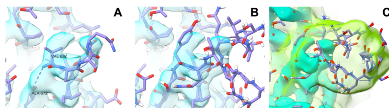
Figure 3. Errors in the experimental model can confound naïve loop modeling approaches. (A) In PDB: 6VSB, residues 673–686 were missing, and residues 687–689 were incorrectly modeled forming the appearance of a severely truncated hairpin. Initial attempts at automated modeling of this loop generated numerous clashes and extremely strained geometry. (B) Manual rebuilding into the high-resolution density showed that the space originally modeled as Val687 actually belongs to Tyr674. (C) While the remainder of the loop was not visible in the high-resolution details of the map, the application of strong Gaussian smoothing revealed a clear envelope, suggesting that the hairpin is capped by short \alpha -helix spanning residues 680–685. The map shown in cyan is as-deposited and contoured at 15\sigma (all panels), and the green map in (C) is smoothed with a B -factor of 100 \text{ \AA}^2 and contoured at 5\sigma . All images were generated using UCSF ChimeraX. 30
