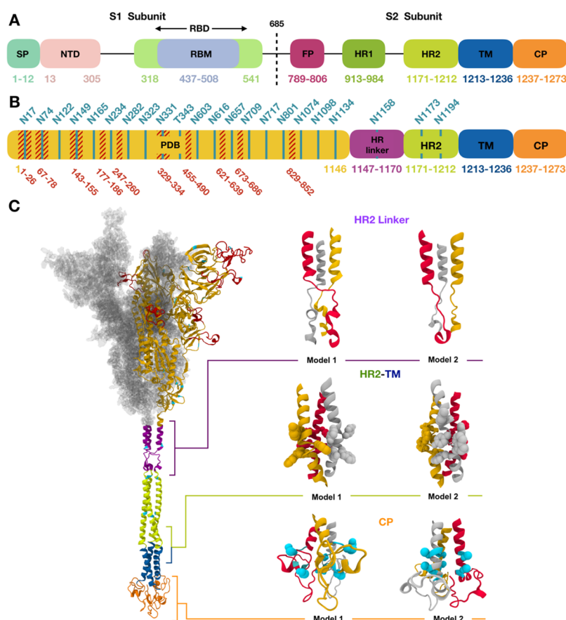
Figure 1. (A) Assignment of functional domains in SARS-CoV-2 S protein: SP, NTD, RBD, receptor binding motif, FP, HR1, HR2, TM, and CP. (B) Assignment of modeling units used for model building. Glycosylation sites are indicated by residue numbers at the top. Missing loops longer than 10 residues or including a glycosylation site in PDB: 6VSB chain A are highlighted in red. Modeled glycosylation sites are shown in cyan. (C) A model structure of full-length SARS-CoV-2 S protein is shown on the left panel using the domain-wise coloring scheme in (B). For the PDB region, only one chain is represented by a secondary structure, while the other chains are represented by the surface. Two models selected for each HR linker, HR2-TM, and CP domain are enlarged on the right panel of (C). Trp and Tyr in HR2-TM are shown in spheres, which are key residues placed on a plane to form interactions with the lipid head group. For CP domain models, the Cys cluster is known to have high probabilities of palmitoylation. Cys1236 and Cys1241 for model 1 and Cys1236 and Cys1240 for model 2 are selected for palmitoylation sites in this study and are represented as cyan spheres. Illustration of S proteins was generated using VMD. 14
