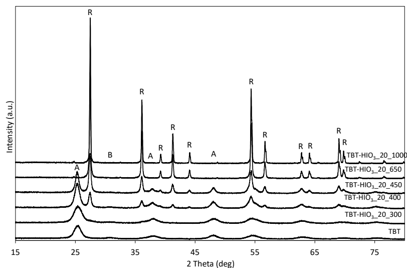
Figure 16. XRD patterns for defective \text{TiO}_2\text{-HIO}_3\text{-T} photocatalysts (A—anatase, B—brookite, and R—rutile).
