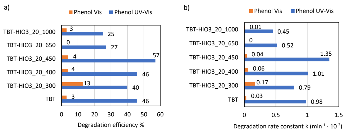
Figure 19. Efficiency of phenol degradation in UV-Vis and Vis light for defective TiO 2 -HIO 3 _20_T photocatalysts, presented as % of degradation (a) and rate constant k (b).
