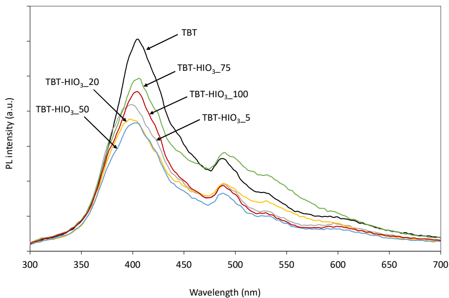
Figure 10. Photoluminescence (PL) spectra for defective \text{TiO}_2\text{-HIO}_3 samples.
