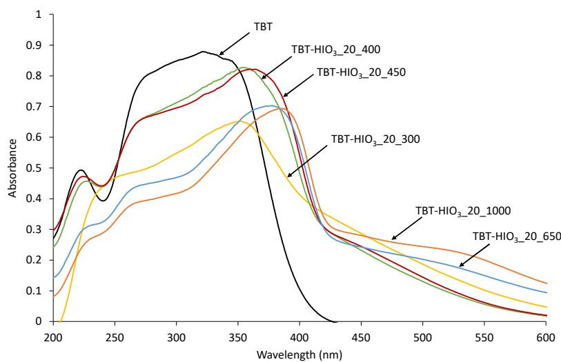
Figure 17. UV-Vis diffuse spectra for pure \text{TiO}_2 and defective \text{TiO}_2\text{-HIO}_3\text{-20-T} photocatalysts calcined in different temperatures.
