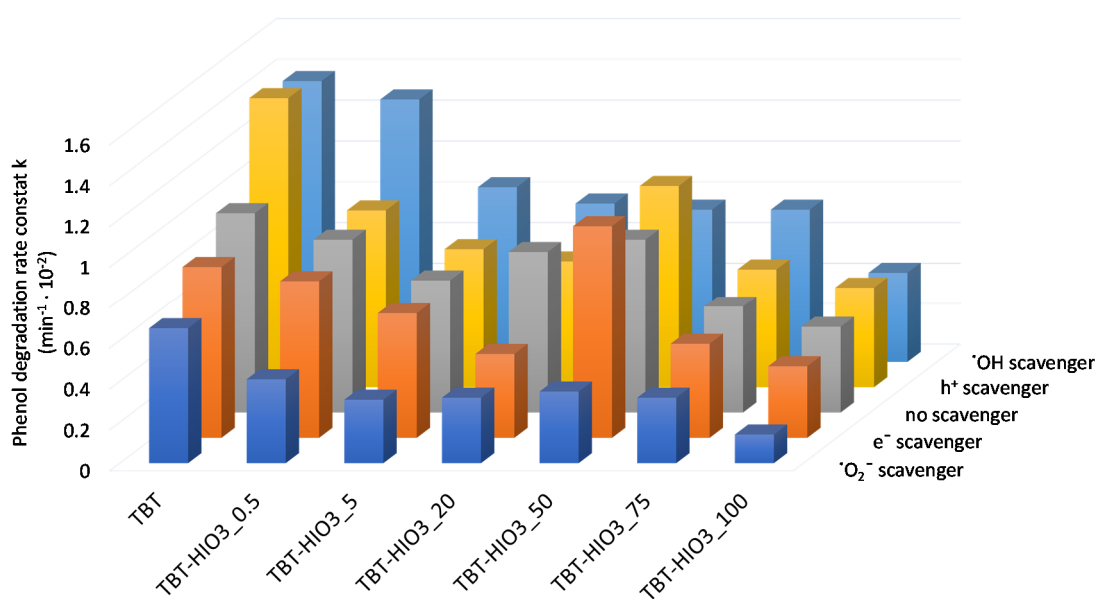
Figure 14. UV-Vis photocatalytic degradation of phenol for \text{TiO}_2\text{-HIO}_3 photocatalyst in the presence of e^- , h^+ , \bullet\text{O}_2^- , and \bullet\text{OH} scavengers.
