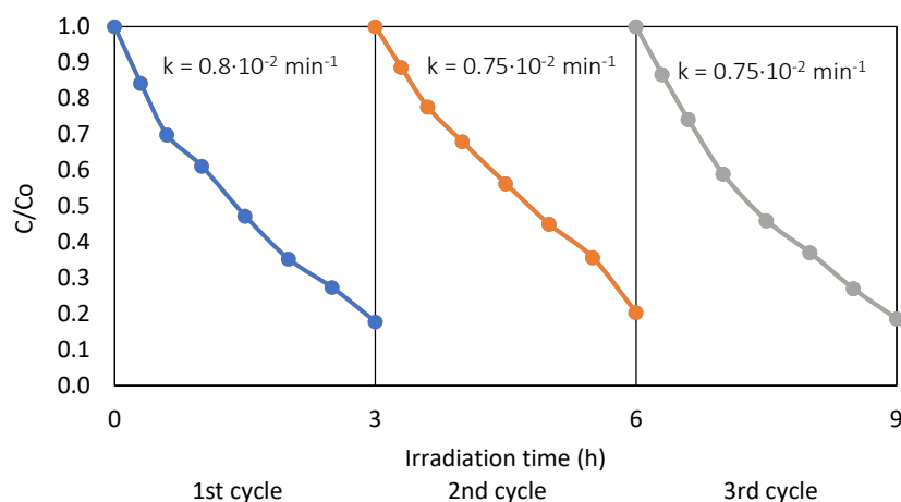
Figure 15. Efficiency of UV-Vis phenol degradation in the presence of a defective TBT- \text{HIO}_3_{50} photocatalyst measured in the three subsequent cycles.
