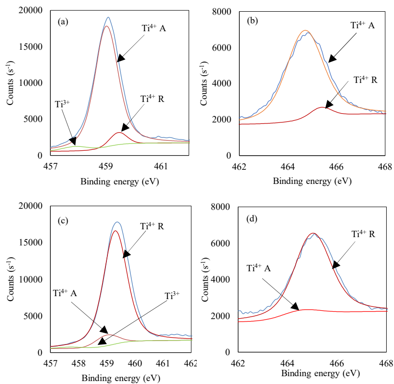
Figure 11. Deconvolution of X-ray photoelectron spectroscopy (XPS) spectra for \text{Ti } 2p_{3/2} and 2p_{1/2} for \text{TBT-HIO}_3_{20} (a,b) and \text{TBT-HIO}_3_{100} (c,d).
