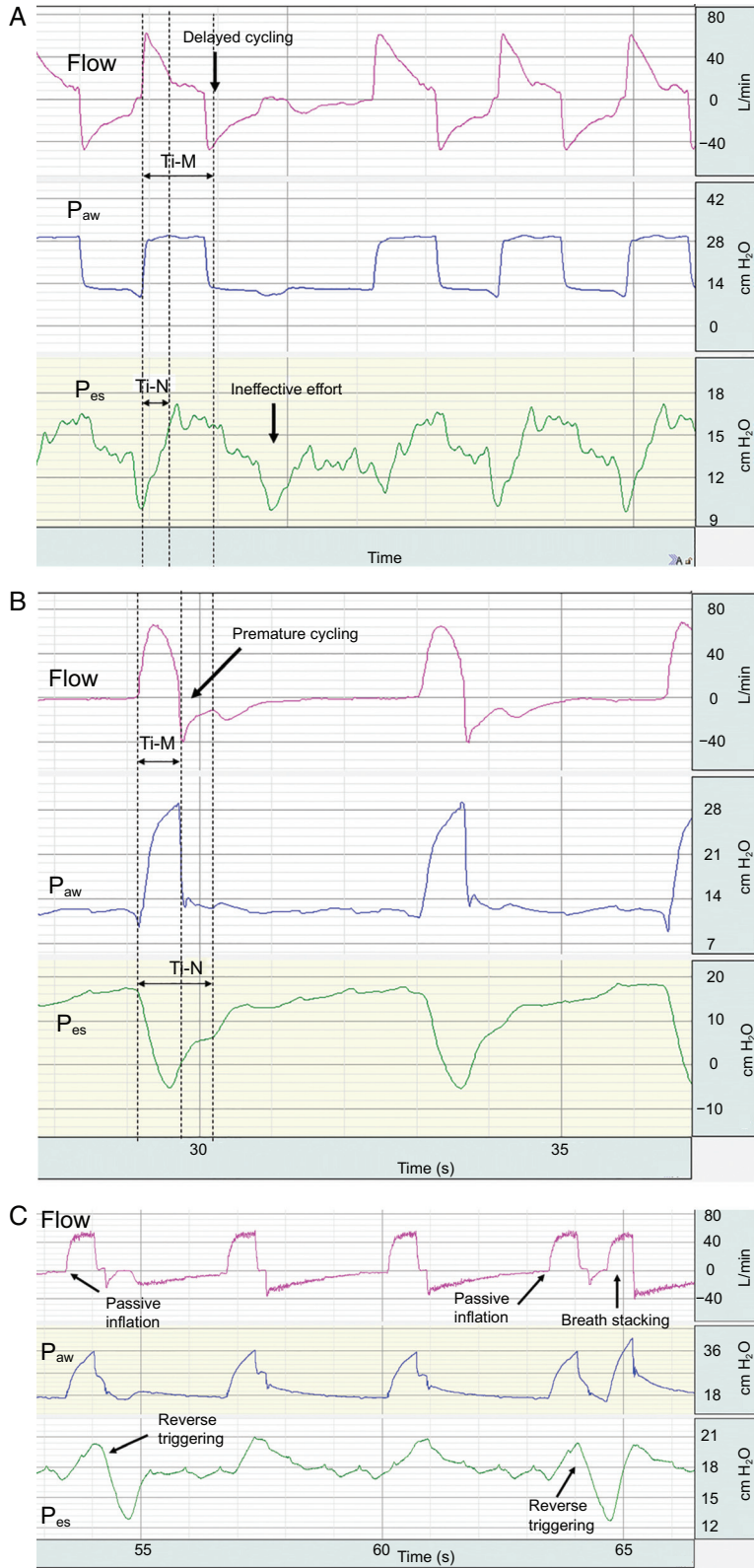
Fig. 6. Flow (pink), airway pressure (P aw , blue), and esophageal pressure (P es , green) waveforms showing patient-ventilator dyssynchronies. (A) In pressure assist controlled mode, the machine inflation time (Ti-M) lasts longer than the patient's neural inspiration (Ti-N), creating delayed cycling. This excess assistance causes ineffective effort in the following breath because the patient's respiratory muscle contraction is not strong enough to trigger an inflation (ie, wasted effort). This is clearly seen on the P es tracing, which shows a negative deflection failing to trigger a
