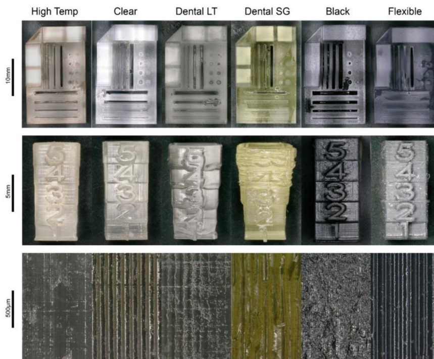
Figure 1. Results of the 3D prints of the photopolymers High Temp, Clear, Dental LT, Dental SG, Black, and Flexible. Top: test print for evaluation of the reproducibility of printing complex features. Centre: test print for evaluation of the level of detail. Bottom: optical enlargement of the surface structure of the different photopolymers.
