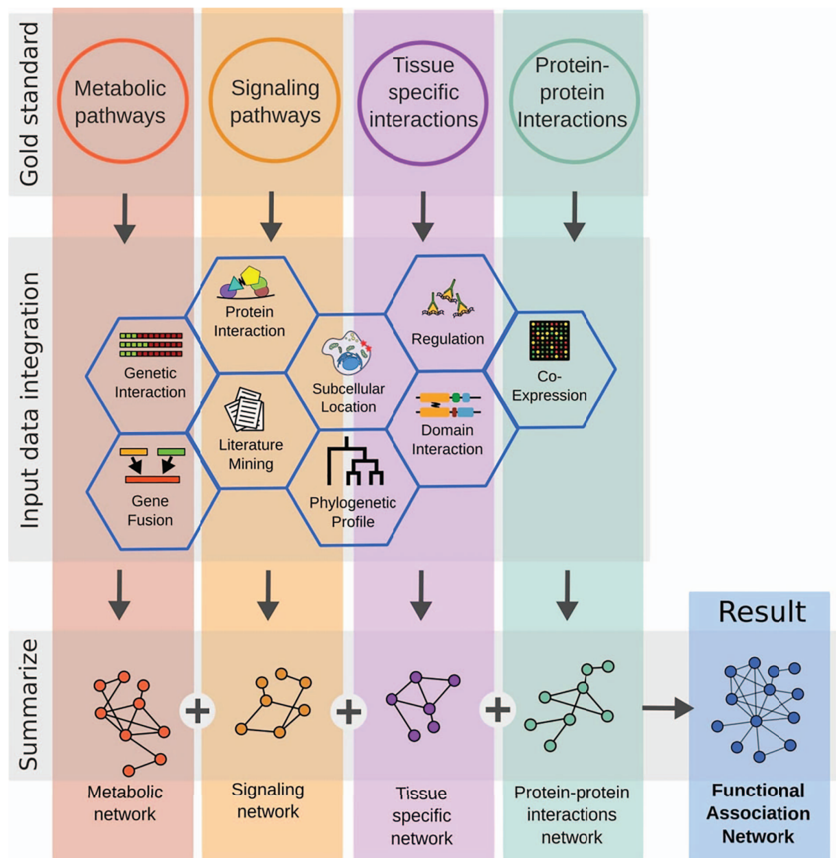
Figure 2. Example workflow to infer a functional association network. All supervised inference methods use a diverse collection of gold standard set. These sets represent known interactions between genes or protein. For example, proteins that physically interact or genes that are present in the same tissue or pathway. Once these homogeneous sets are defined, they can be applied separately as labels to an assemblage of input data spanning from co-expression over domain interaction to phylogenetic profiles. The labeled data are further used to train supervised methods and predict interactions between genes that have been not known so far. Each prediction is still specific to the gold standard used for labeling the data to begin with. To increase the power and coverage most methods summarize all networks in an ensemble network, incorporating all interaction types. Since the interaction loses its gold standard specific meaning it is newly defined as functional association.
