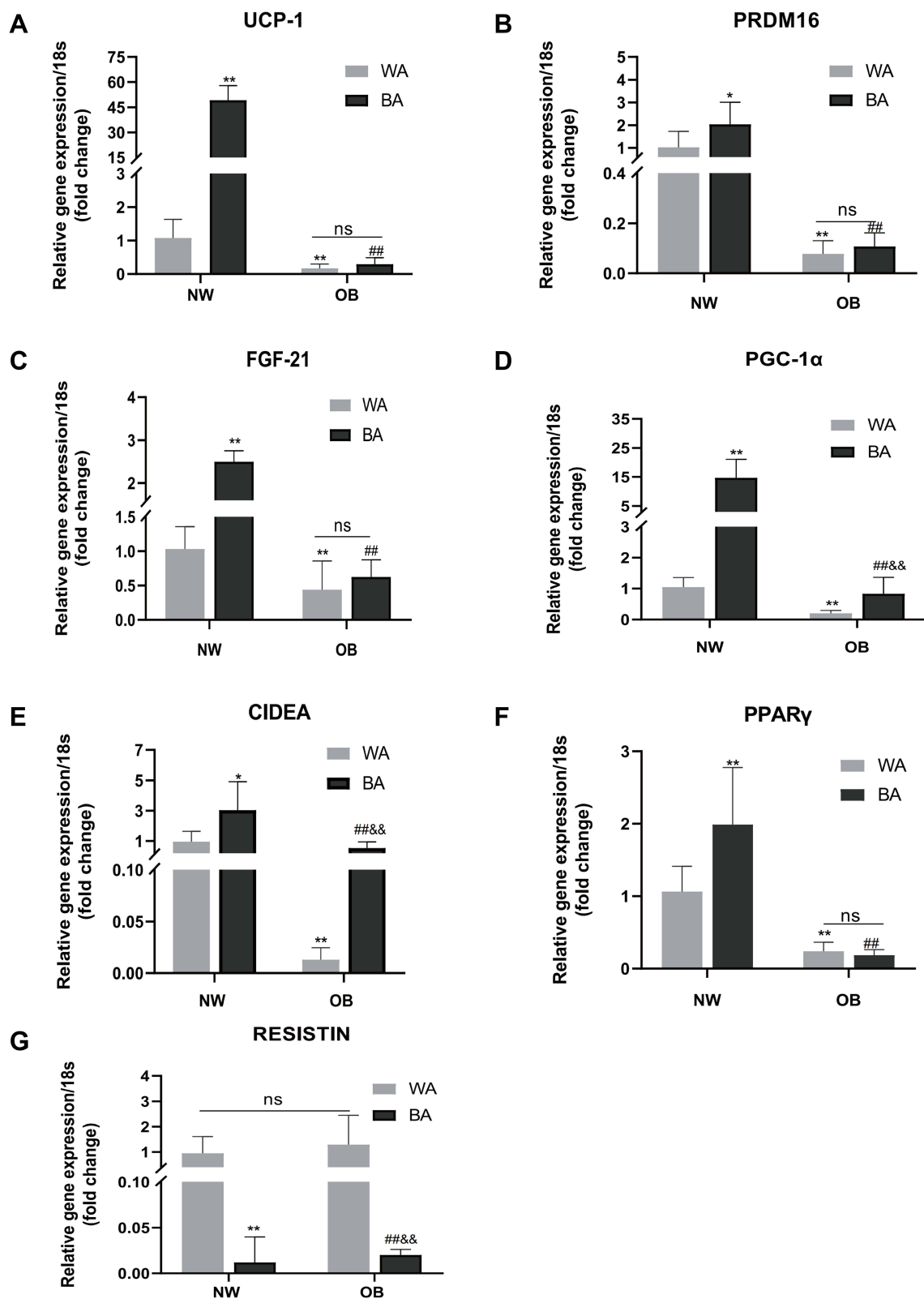
Figure 3 Thermogenic and adipogenic genes expressions in differentiated adipocytes. Comparison of UCP-1 (A), PRDM16 (B), FGF21 (C), PGC-1 \alpha (D), CIDEA (E), PPAR \gamma (F) and resistin (G) mRNA expressions of WA- and BA-induced adipocytes in normal-weight (NW) and obese (OB) groups. Values are mean \pm SD; n=12 for NW-WA, NW-BA, OB-WA and OB-BA groups; data used for analysis were mean values of three replicate experiments for each sample; * p < 0.05 vs NW-WA group, ** p < 0.01 vs NW-WA group, *** p < 0.01 vs NW-BA group, ** p < 0.01 vs OB-WA group. Abbreviation: ns, not significant.
