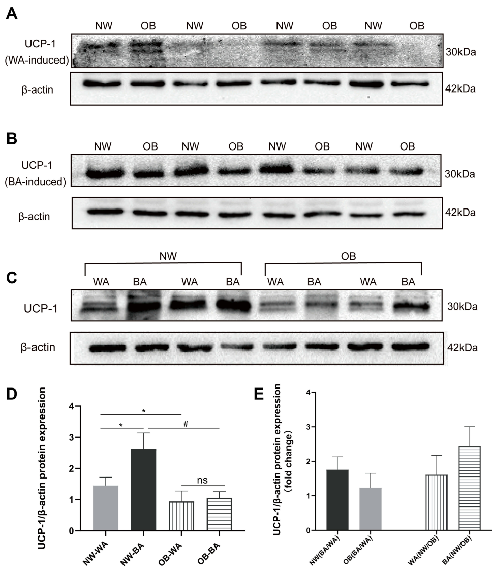
Figure 4 UCP-1 protein expression in differentiated adipocytes. Western-blot images of UCP-1 protein band density of normal-weight group (NW) and obese (OB) group in WA (white adipocyte)-induced ( A ) and BA (beige adipocyte)-induced ( B ) adipocytes, and UCP1 protein band density of WA- and BA-induced adipocytes from the same adipose tissue sample in NW and OB group ( C ). ( D ) The analysis of UCP-1 protein band values in NW-WA, NW-BA, OB-WA and OB-BA groups. ( E ) Fold changes of UCP-1 protein expression in NW and OB group with WA- and BA-induction treatment. Values are mean \pm SD; n = 12 for NW-WA, NW-BA, OB-WA and OB-BA groups; * p < 0.01 vs NW-WA group, # p < 0.01 vs NW-BA group.
