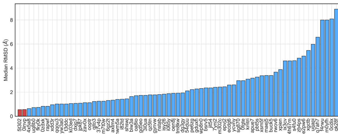
Figure 6: Performance comparison of different submissions on pose prediction challenge of Stage 1a for the BACE dataset in term of median RMSD. Our submissions are highlighted in the red color, in which the best one is 5t302 with median RMSD = 0.55 Å.
