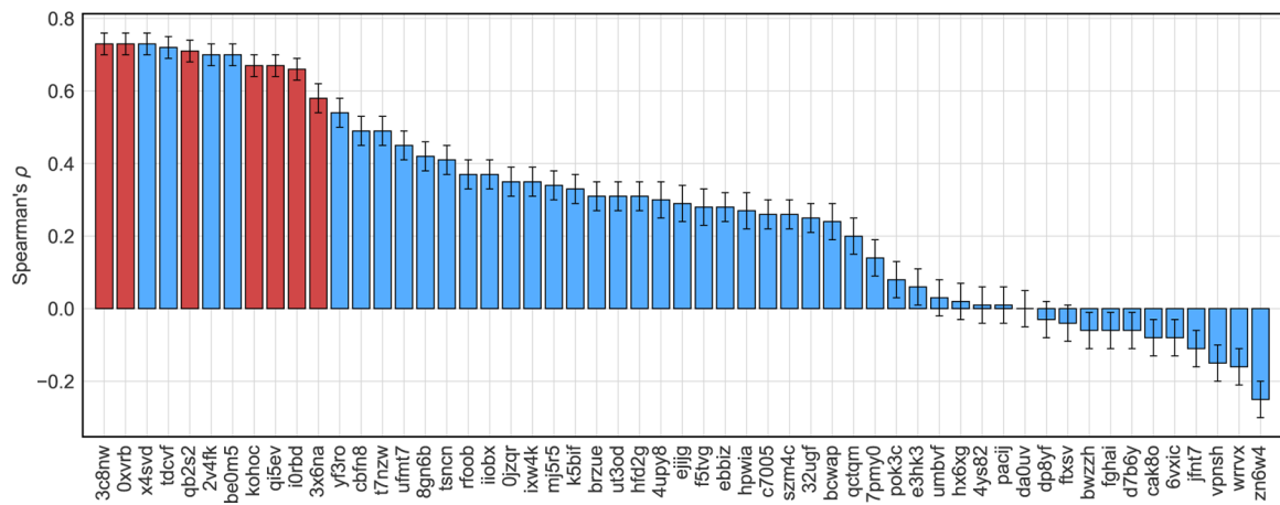
Figure 8: Performance comparison of different submissions on the combined ligand and structure based scoring of CatS dataset in term of Spearman's \rho . Our submissions are highlighted in the red color, in which our top-ranked submissions are 3c8nw and 0xvrb with \rho=0.73 .
