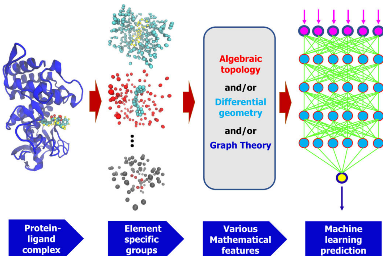
Figure 4: A framework of MathDL energy prediction model which integrates advanced mathematical representations with sophisticated CNN architectures
