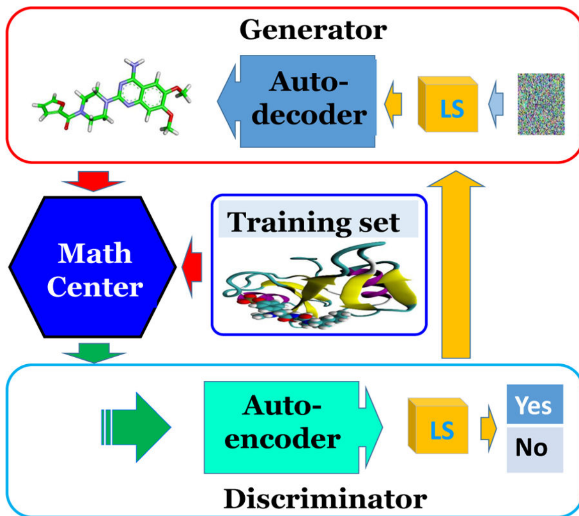
Figure 5: Illustration of our docking approach using mathematical representations integrated with GAN architectures. The generator contains an autodecoder, a latent space (LS), and a noise source. The discriminator consists of an autoencoder and latent space. The Math center encodes 3D structures into low-dimensional mathematical representations using algebraic topology, differential geometry, and/or graph theory.
