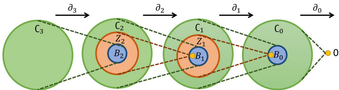
Figure 3: Illustration of boundary operators, chain, cycle, and boundary groups in \mathbb{R}^3 . Yellow circles are empty sets.
