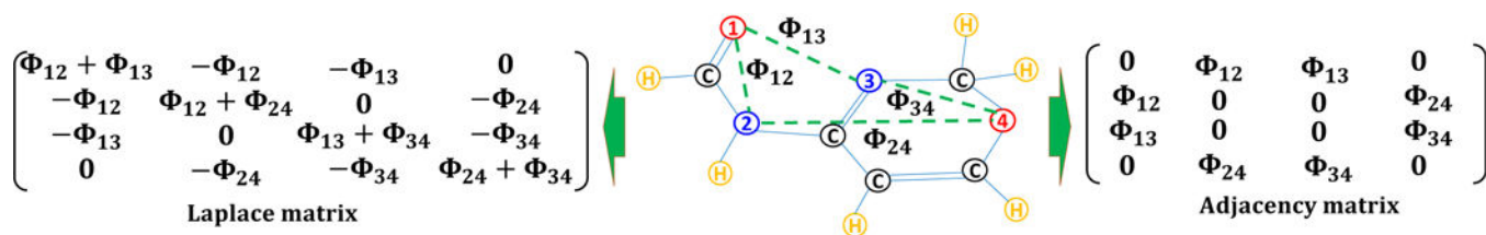
Figure 2: Illustration of weight colored subgraphs G_{NO} including its Laplacian matrix (Left), and adjacency matrix (Right) deduced from molecule graph ( C_5H_6N_2O_2 ) (Middle). Atoms 1 and 4 are oxygen, while atoms 2 and 3 are nitrogen. Graph edges, \Phi_{ij} , are in the green-dashed lines representing the noncovalent bonds. In addition, one can get 9 other nontrivial subgraph for this molecule, namely G_{CC} , G_{CN} , G_{CO} , G_{CH} , G_{NN} , G_{NH} , G_{OO} , G_{OH} , and G_{HH} .
