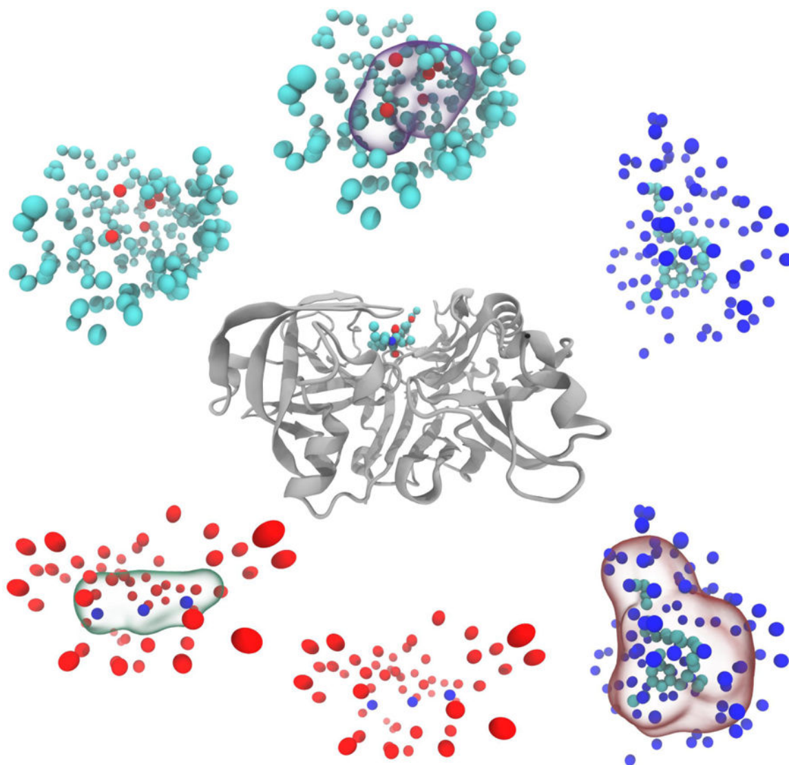
Figure 1: Illustration of some element-specific selections and corresponding element interactive manifolds obtained at a given level set of the element interactive density. Each sphere illustrates the atomic positions. Cyan, red, and blue colors represent carbon, oxygen, and nitrogen, respectively. The transparent surfaces are the isosurface extracted from volume data represented in Eq. (8).
