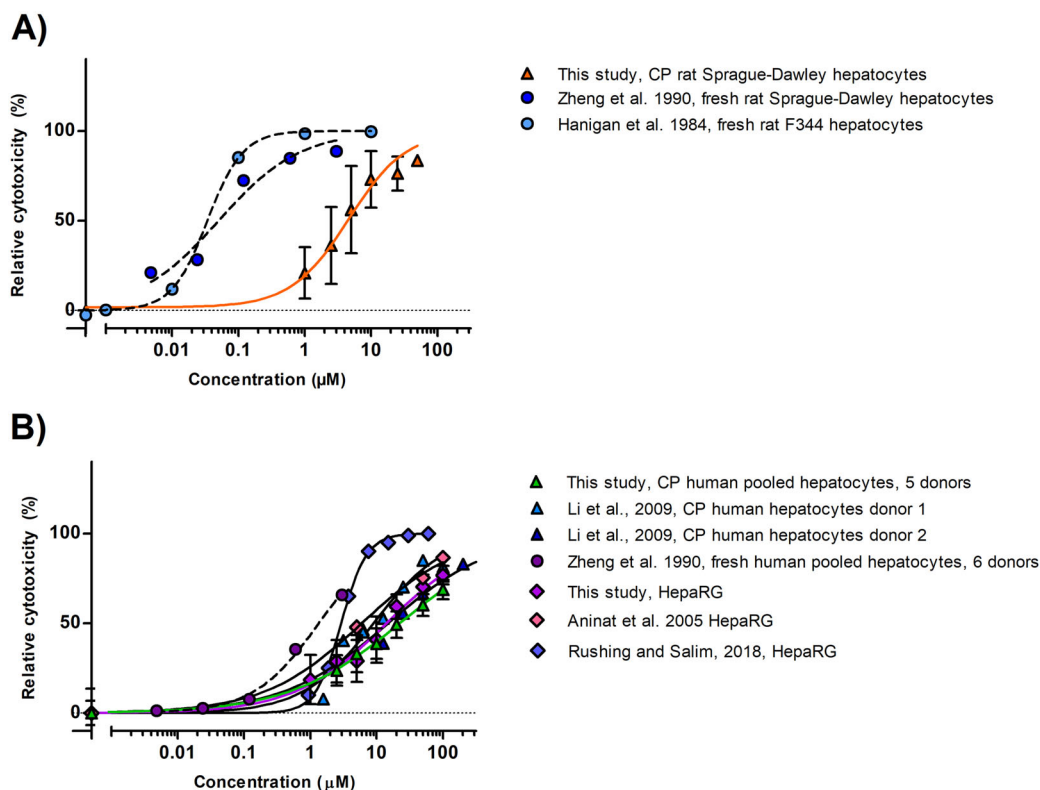
Figure 2. Concentration response curves for the cytotoxicity of AFB1 ( \mu\text{M} ) in A) rat and B) human cell models upon 24 h exposure in medium without serum (mean values + SD) as measured in the present study and reported in literature. Circle symbols with dotted curves correspond to fresh hepatocytes. Triangle symbols to cryopreserved hepatocytes, and diamonds to HepaRG cells. CP: cryopreserved.
