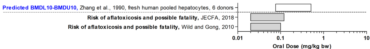
Figure 7. Predicted BMDL10-BMDU10 values for acute liver toxicity of AFB1 in human obtained by the PBK modeling-facilitated reverse dosimetry approach using data from fresh human hepatocytes. [54] The predicted BMDL10-BMDU10 (white rectangle bars) are compared to the estimated doses that can cause a risk of acute aflatoxicosis and possibly fatality in humans [4,9] (gray rectangle bars).
