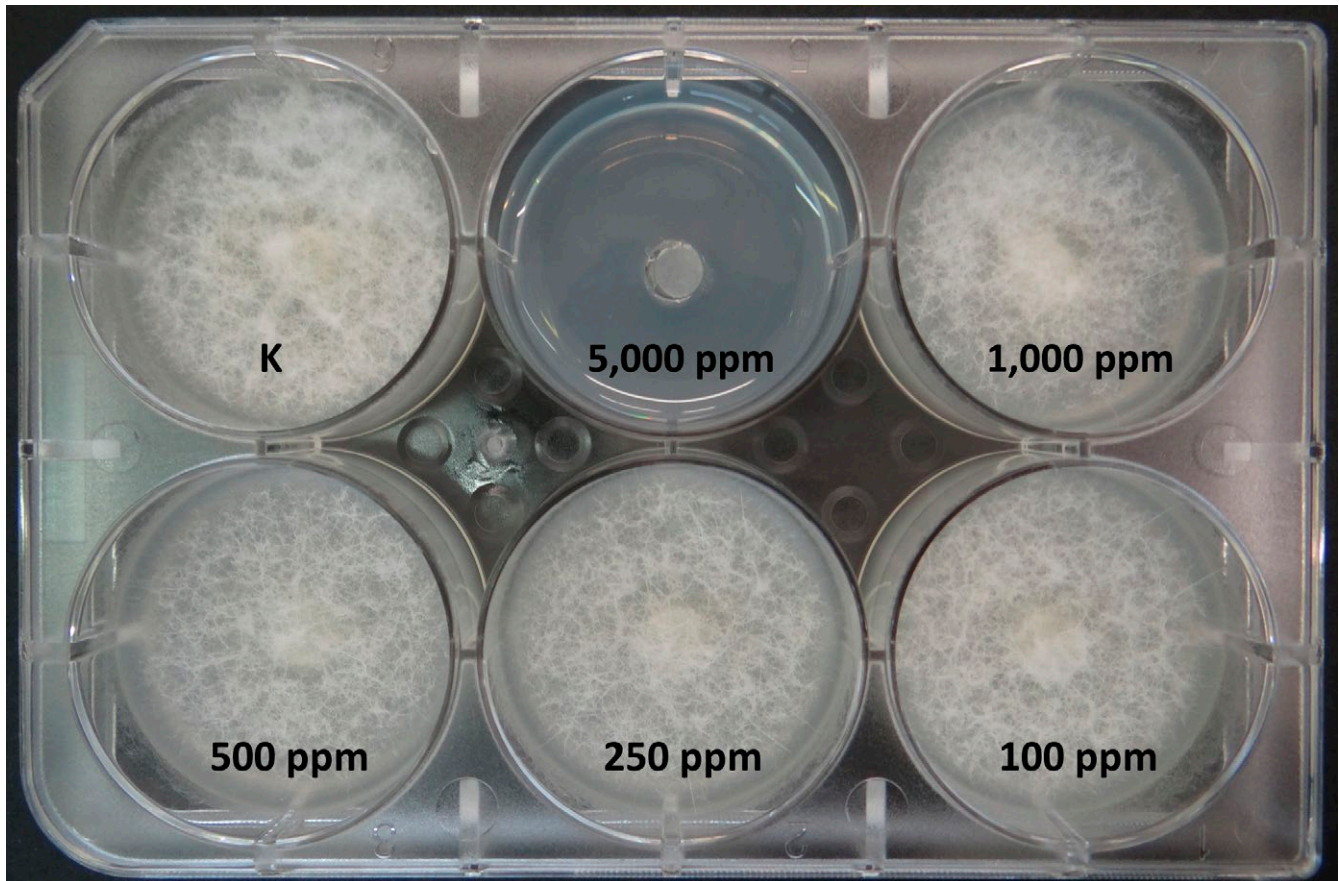
FIGURE 4 Mycelial growth after 6 days with different concentrations of hydrogen peroxide in agar, showing minimum inhibitory concentration at 5,000 ppm [Colour figure can be viewed at wileyonlinelibrary.com ]
