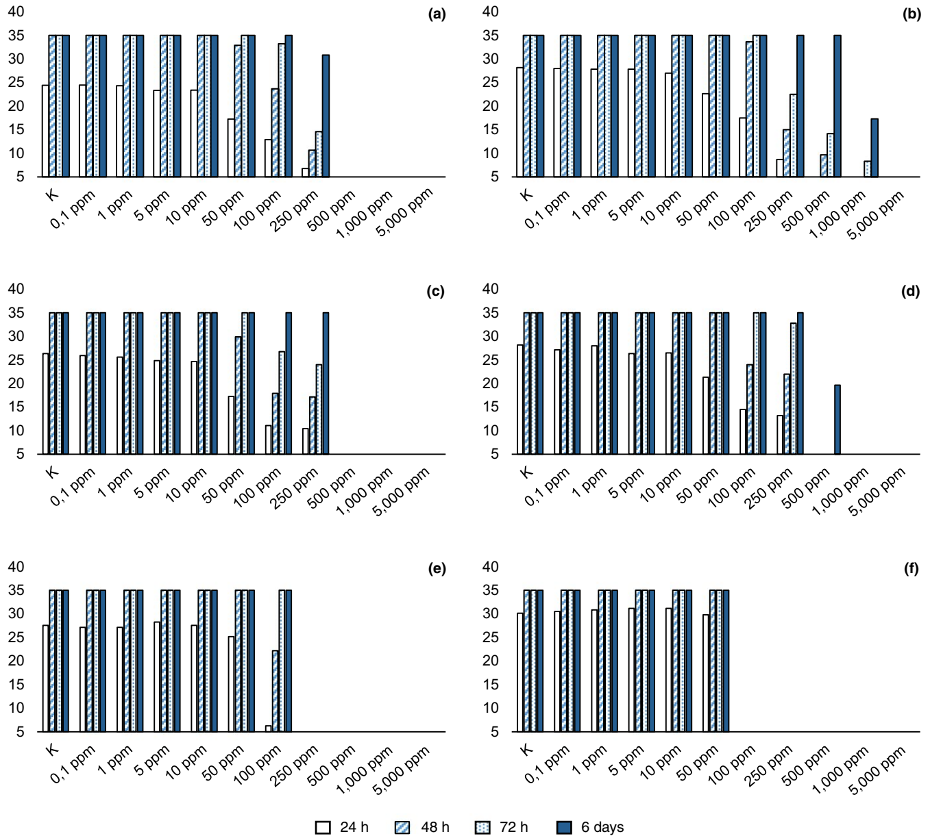
FIGURE 3 Average diameter (mm) of Saprolegnia parasitica and Saprolegnia delica mycelium with different concentrations of compound in agar. (a) S. parasitica , lactic acid; (b) S. delica , lactic acid; (c) S. parasitica , tartaric acid; (d) S. delica , tartaric acid; (e) S. parasitica , iodoacetic acid; (f) S. delica , iodoacetic acid [Colour figure can be viewed at wileyonlinelibrary.com ]
