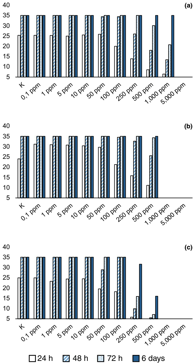
FIGURE 5 Average diameter (mm) of mycelium with different concentrations of product in agar. (a) Actidrox; (b) Detarox; (c): Virkon [Colour figure can be viewed at wileyonlinelibrary.com ]
