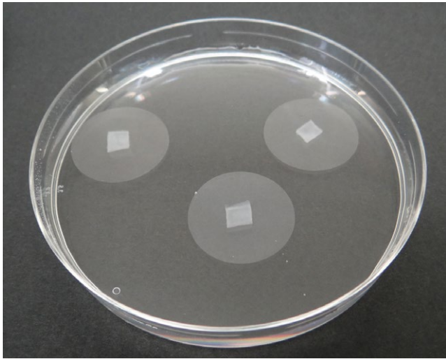
FIGURE 1 Protocol II: Filters supporting mycelium immersed in a solution of the product under test [Colour figure can be viewed at wileyonlinelibrary.com ]
