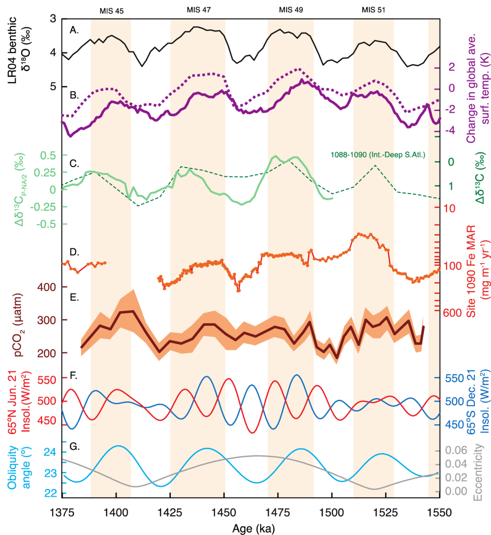
Figure 4. Boron-based pCO 2 record compared with orbital-scale records of the early Pleistocene climate. (A) LR04 benthic oxygen isotope stack [black, Lisiecki and Raymo , 2005] reflects high-latitude temperature and ice volume changes on the dominant ~41-kyr ice age cycle during this interval. (B) Compilations of sea surface temperature records used to estimate change in global average surface temperature (dashed line from Martínez-Botí et al. [2015a] and solid line from Snyder [ Snyder , 2016]). (C) Benthic carbon isotope gradients between Pacific and North Atlantic basins (solid light green line, \delta^{13}\text{C}_{\text{Pacific}-(\text{North Atlantic})/2} ) [ Lisiecki , 2010] and between intermediate and deep water in the south Atlantic (dashed line) [ Hodell and Venz-Curtis , 2006]. (D) Marine accumulation rate of Fe from ODP Site 1090 (solid line) [ Martínez-García et al. , 2011]. (E) Calculated \delta^{11}\text{B} -based surface ocean pCO 2 from Figure 3. (F, G) Summer insolation at 65°N (blue) and 65°S (red) and orbital parameters [ Laskar et al. , 2004].
