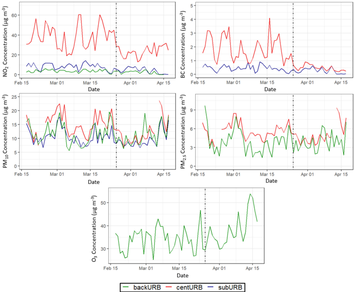
Fig. 4. Daily 24-hour average time-series concentrations for \text{NO}_2 , \text{O}_3 , \text{PM}_{10} , \text{PM}_{2.5} & BC at the subURB (blue), centURB (red) & backURB (green) sites between 17 February 2020–17 April 2020. The lockdown date is indicated by the black dashed line (27 March 2020).
