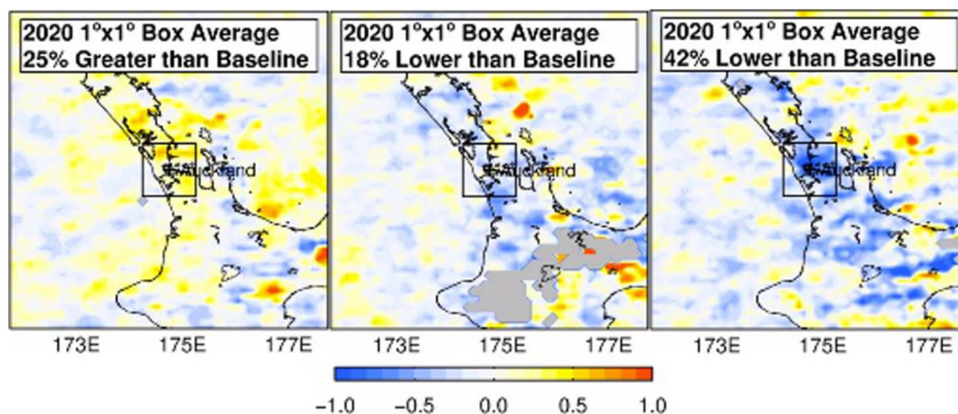
Fig. 7. Median \text{NO}_2 anomaly ( \times 10^{15} molec. \text{cm}^{-2} ) based on 2015–2019 running median for 17th February 2020 (left), 26th March 2020 (middle) & 17th April 2020 (right) (NASA, 2020).
