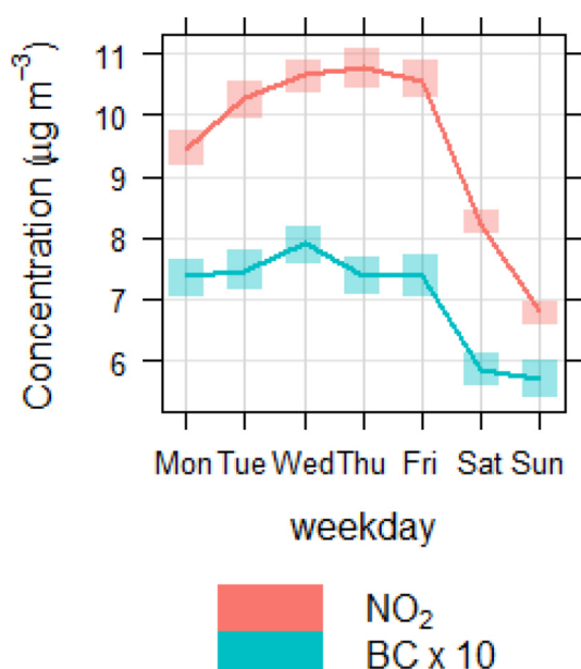
Fig. 8. Historical (2015–2020) day-of-week \text{NO}_2 & BC concentrations from the subURB site.
