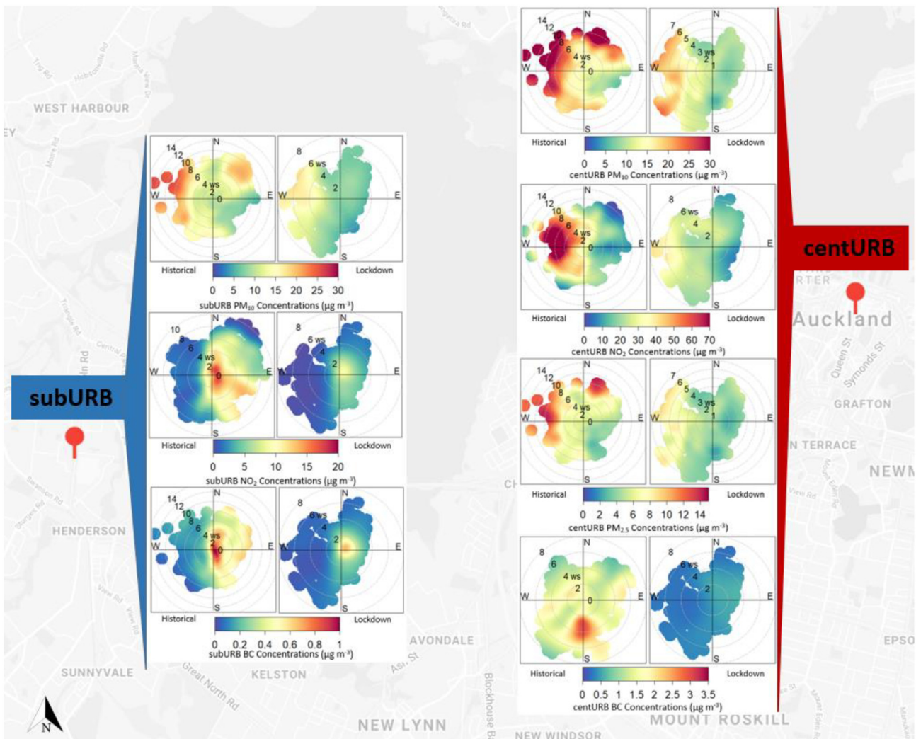
Fig. 9. Polar plots of PM 10 , NO 2 & BC at the subURB site (left) and polar plots of PM 10 , PM 2.5 , NO 2 & BC at the centURB site (right) site during historical (February, March & April 2016–2020) and lockdown (26th March 2020–17th April 2020) periods.
