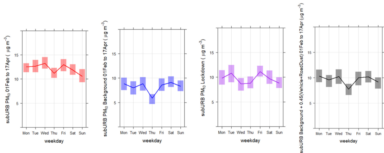
Fig. 12. Weekday PM_{10} at the suburb site; (a) Historical PM_{10} concentrations for Feb–April, (b) Estimated background PM_{10} from receptor modelling, (c) PM_{10} concentrations during lockdown (d) estimated PM_{10} during lock down that includes background plus 45% of the motor vehicle and road dust component. The dark lines indicate the mean concentrations with 95% confidence (shaded areas).
