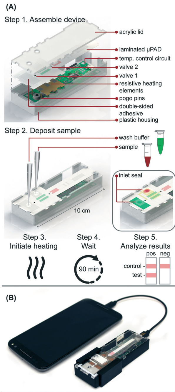
Figure 1. (A) Schematic of microRAAD for HIV testing work flow in which user 1) assembles consumable \mu PAD into plastic housing with reusable resistive heating elements and heating control board, 2) deposits sample and wash buffer into inlets and seals with tape to minimize evaporation, 3) initiates heating by connecting to phone, 4) waits 90 minutes for automated fluid delivery and sample incubation in \mu PAD, and 5) analyzes results of lateral flow immunoassay. (B) Photo of microRAAD connected to phone to power the heating control board.
