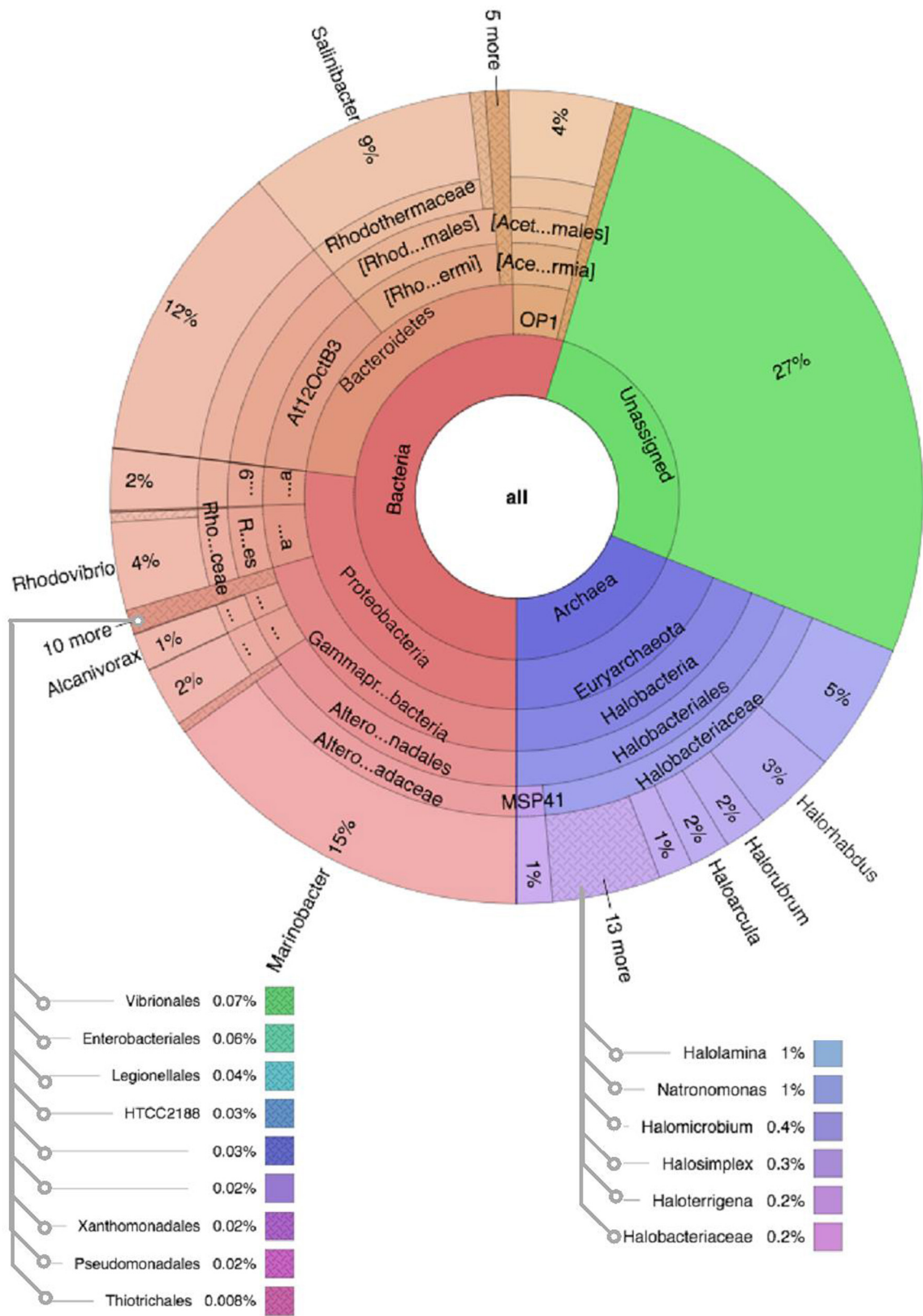
FIGURE 5 | Multivariate OTU clusters of Karak salt samples. Legends: Archaea (blue), Unassigned (green), and Bacteria (Red/Orange), with lighter shades signifying lower taxonomic levels (toward species-level).
