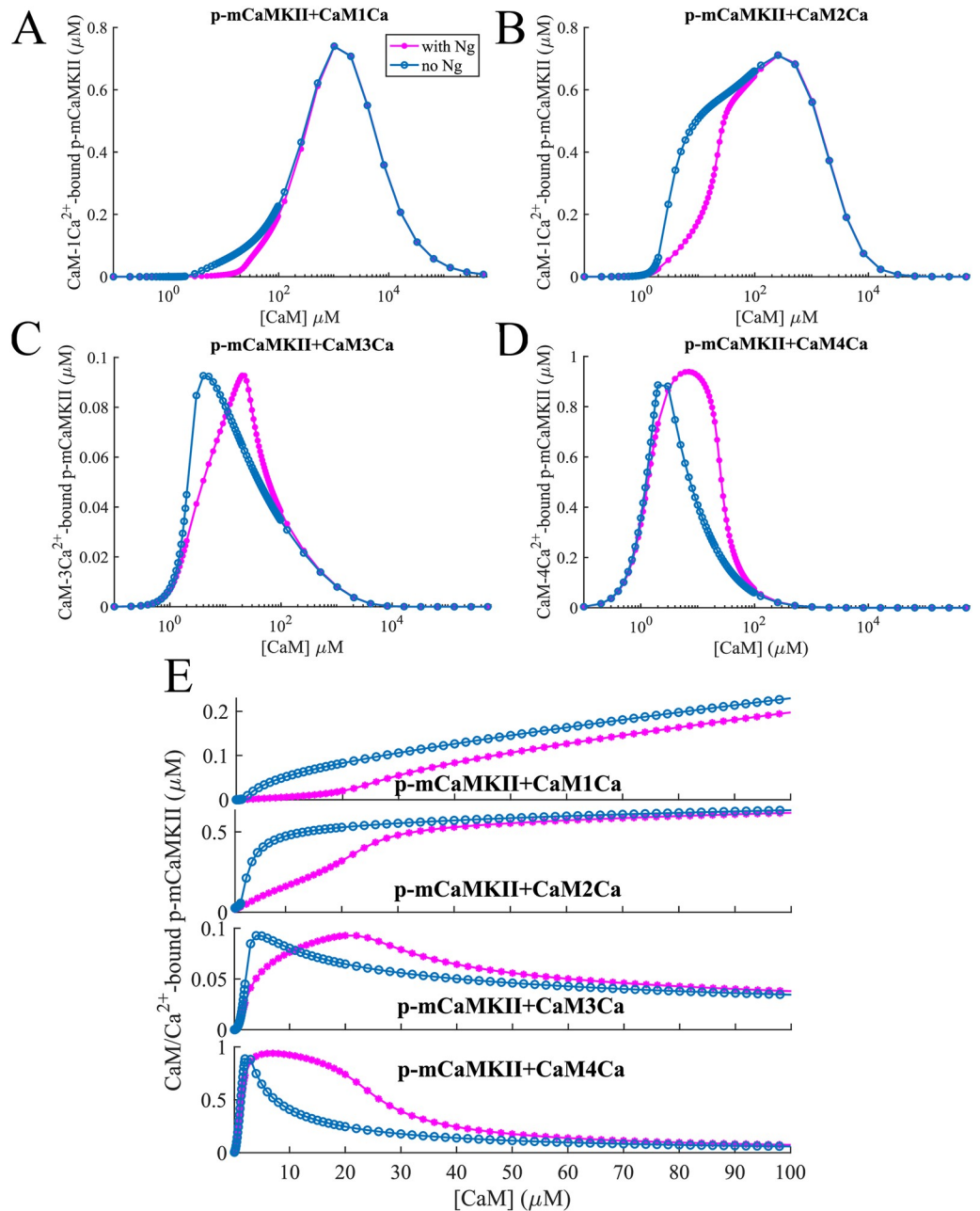
Fig 3. mCaMKII phosphorylation. Dose response of phosphorylated mCaMKII molecules bound to (A) 1-, (B) 2-, (C) 3- and (D) 4-calcium states of CaM-Ca 2+ as shown in Fig 2. At low [CaM], the “multi-calcium-bound” forms of calmodulin play an important role. This is amplified by the fact that these forms when bound to CaMKII give it higher phosphorylation rates (Table 1). (E) shows the same effect for physiologically relevant [CaM]. In these simulations, input [Ca 2+ ] = 10 μM constant.
