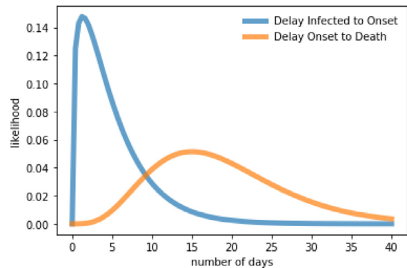
Fig. 2. Illustration of probability density functions for d_{iso} and d_{iso-death} used in the current study. The parameters of the distributions are used from [11].
