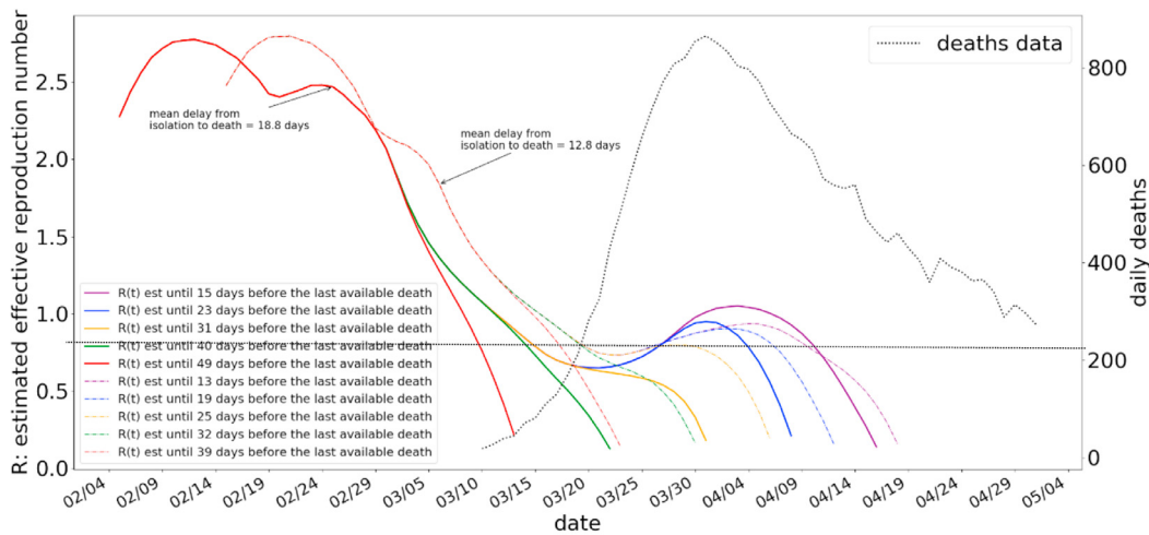
(b) R estimation from the proposed method and the number of deaths reported.
