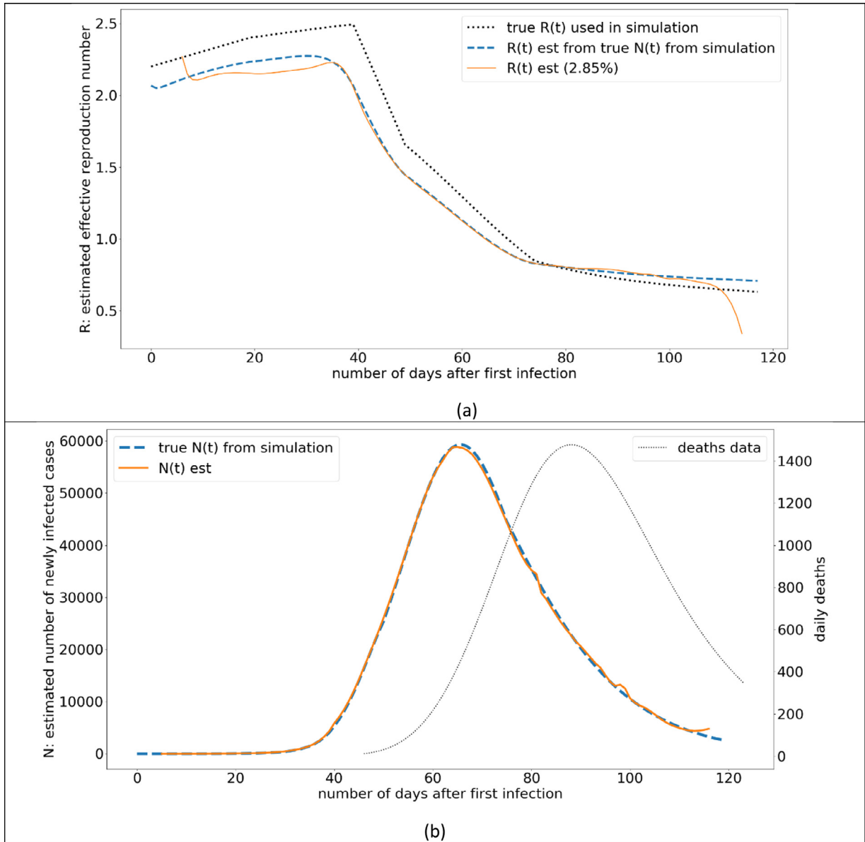
Fig. 3. Model Validation: (a) The variation of simulated R(t) value, and the R(t) value estimated from the proposed model, (b).
