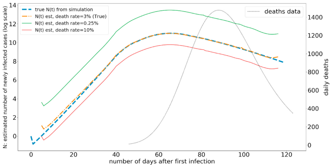
(a) N(t) estimation under different mortality rates
