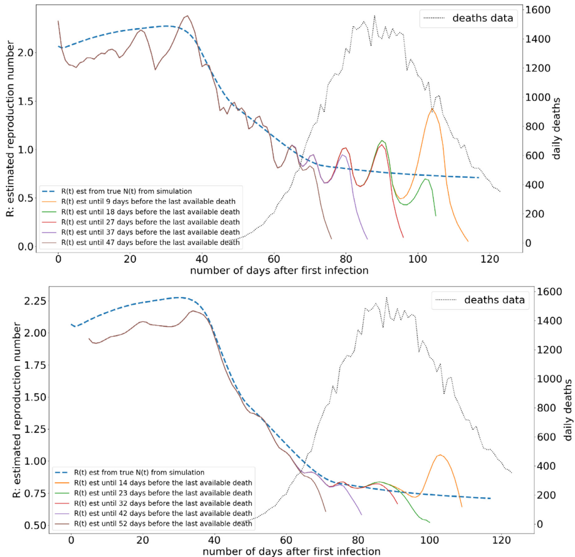
Fig. 8. The variation of R(t) estimation under different gaps from the most recent death data availability. The delay from isolation to death is “assumed” as a gamma distribution with mean = 21.8, and shape = 4.94, the noise level on the death data is 5%.
