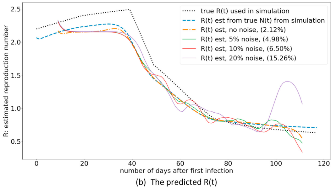
Fig. 6. The variation of R(t) estimation under different noise levels on the death statistics.
