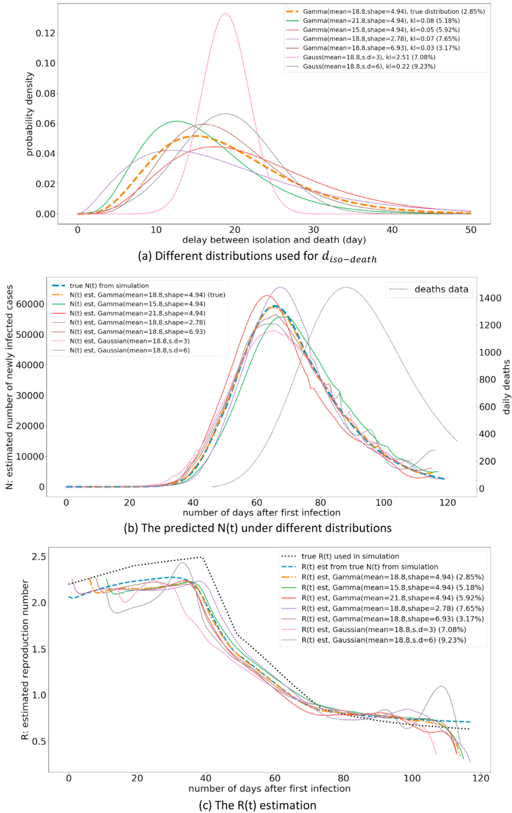
Fig. 4. The variation of R(t) estimation under different d_{iso-death} distributions.
