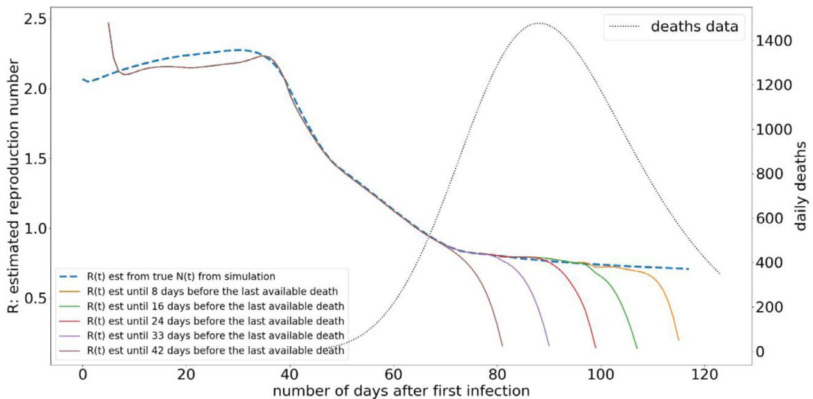
Fig. 7. The variation of R(t) estimation under different gaps from the most recent death data availability. The “true” delay from isolation to death is simulated as a gamma distribution with mean = 18.8, and shape = 4.94, and same distribution used in the method.
