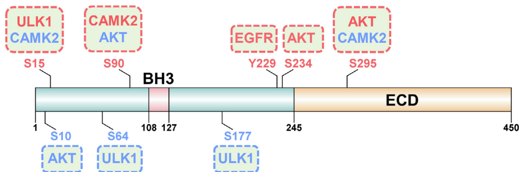
Figure 5 Prediction of kinase-specific p-sites in human Beclin-1
