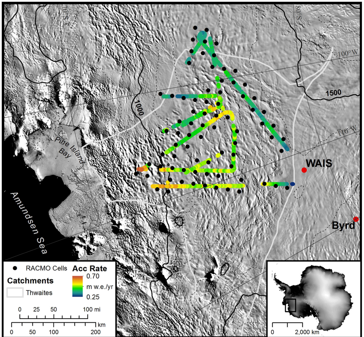
Fig. 2. Map of the study area, including catchment delineation (white line), elevation contours (black lines), radar-derived SMB and the location of the RACMO grid points used for comparison (black dots). The background image is de MODIS Mosaic of Antarctica (Scambos et al., 2007).
