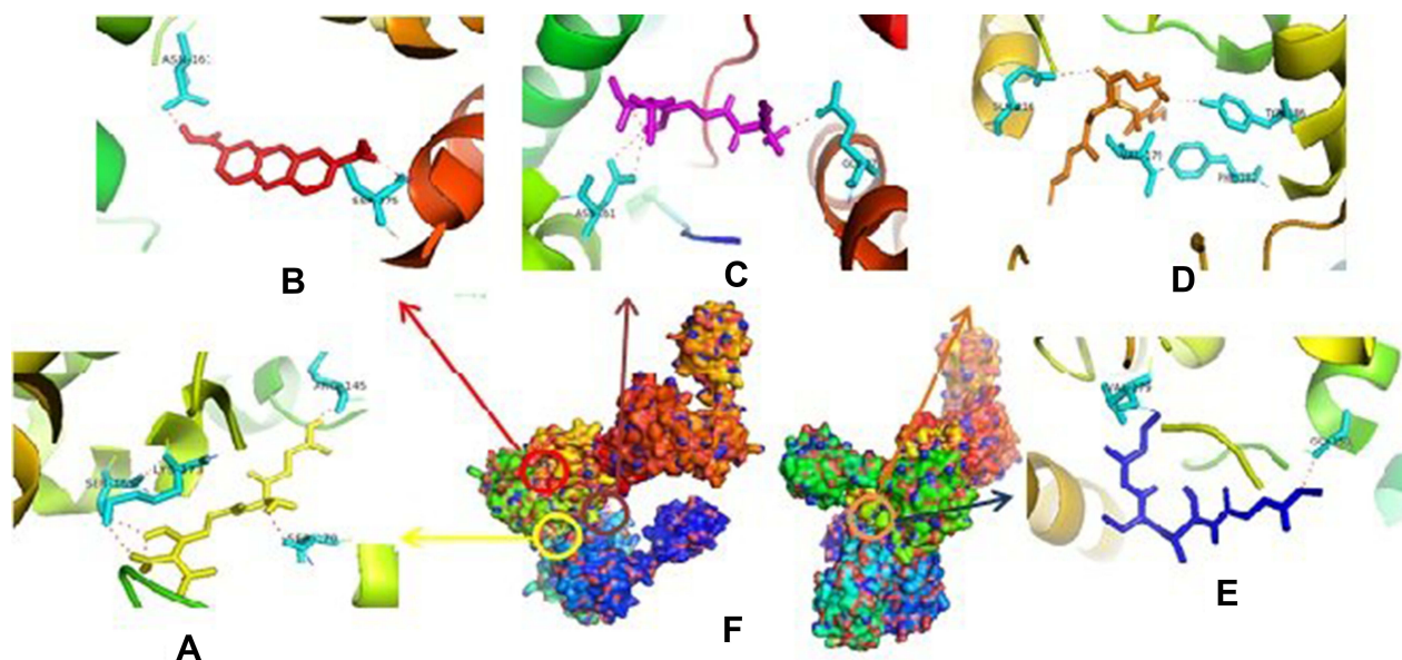
Figure 2 Binding site of amoxicillin (A), compound I (B), ampicillin (C), enalapril (D), esomeprazole (E) against amino acid residue from PrgQ proteins (F).
