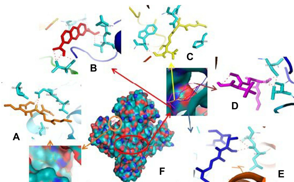
Figure 3 Binding site of enalapril (A), compound I (B), amoxicillin (C), ampicillin (D), esomeprazole (E) against amino acid residue from PrgZ (F) proteins.
