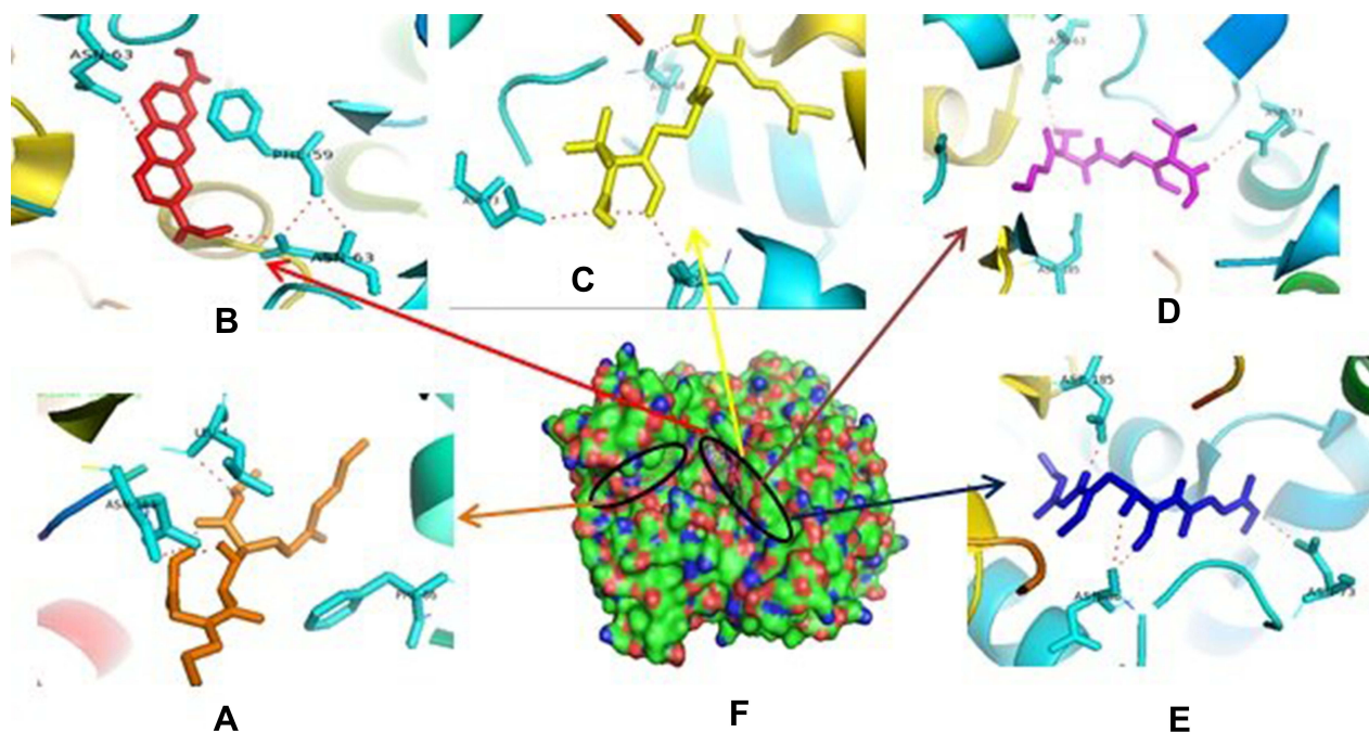
Figure 4 Binding site of enalapril (A), compound 1 (B), amoxicillin (C), ampicillin (D), esomeprazole (E) against amino acid residue from PrgX proteins (F).
