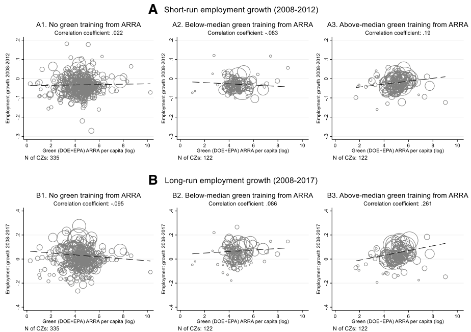
Fig. 1 Green ARRA and Employment Growth: The Role of Training. Notes: 579 Commuting Zones with population > 25 k. DOE+EPA ARRA spending refers to cumulative ARRA spending awarded by the Department of Energy and the Environment Protection Agency over 2009–2012 (Source: FedSpending.org). Employment growth: logarithmic difference in total employment (source: Quarterly Census on Employment and Wages, BLS) between 2012 and 2008 (panel A) and 2017–2008 (panel B). Size of circles is proportional to CZ's population in 2008. Correlation coefficients and linear interpolation are weighted with population in 2008. The median value of ARRA green training per capita for areas with positive funding is $2.6
