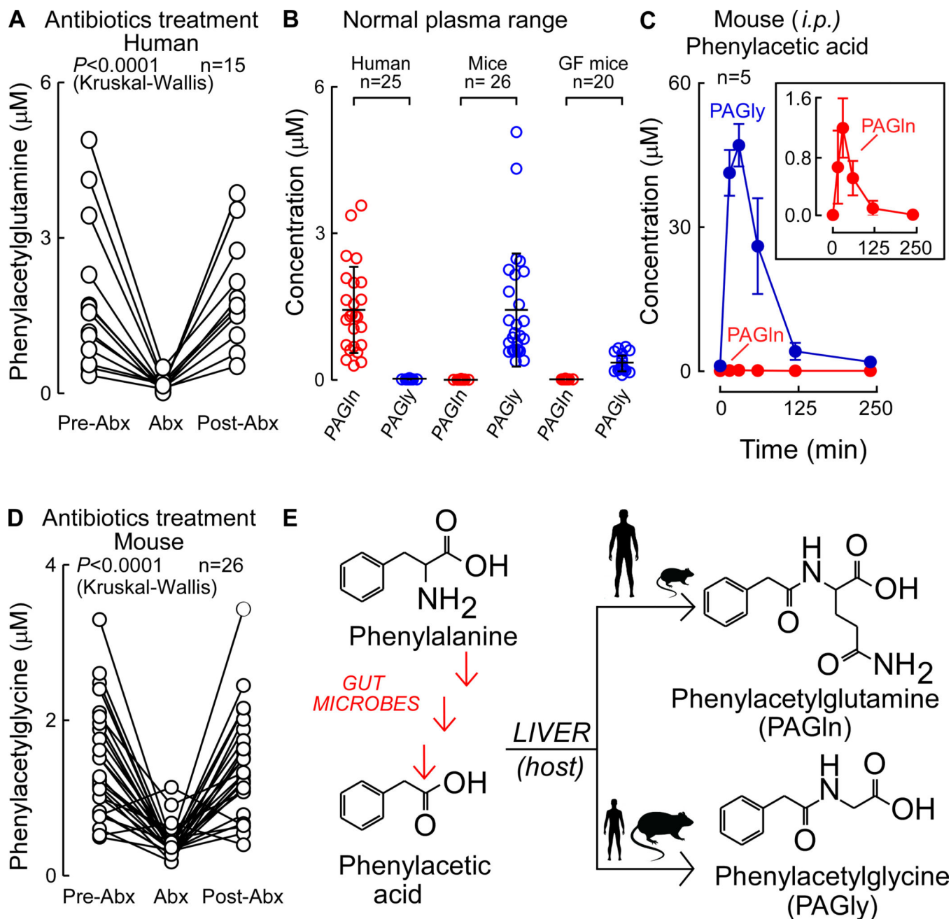
Figure 2. PAGln Production In Vivo is a Microbiota-Dependent Process in Humans and Mice. Fasting plasma levels of PAGln in subjects ( n = 15 ) (i) before oral treatment with a cocktail of poorly absorbable, broad spectrum antibiotics (Pre-Abx), (ii) after seven days of antibiotics regiment (Abx), and (iii) three weeks after discontinuation of antibiotics (Post-Abx). Kruskal-Wallis was used for the statistical analysis. (B) Fasting plasma levels of PAGln and PAGly (mean \pm SD) in indicated numbers of healthy human subjects ( n = 25 ; left), conventionally raised mice ( n = 26 ; mid) and germ free (GF) mice ( n = 20 ; right).
