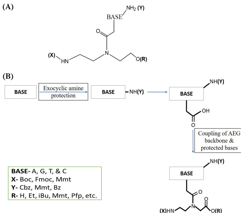
FIGURE 4 (A) General PNA monomer schematic illustration; (B) diagrammatic illustration explaining the synthesis procedure of PNA monomer
