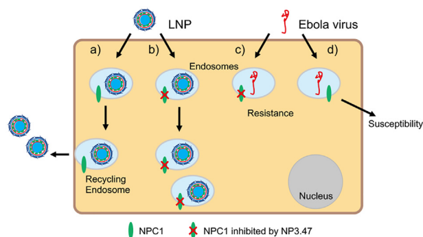
Fig. 8. Mechanisms of enhanced cellular retention of LNPs in cells treated with NP3.47, a NPC1 inhibitor. a) LNPs are often exocytosed to the outside of the cells. b) Endosomal recycling mechanism is impaired by NP3.47 treatment, resulting in enhanced retention of LNPs. c) In cells treated with NP3.47, infection of the Ebola virus is suppressed by inhibiting endosomal recycling mechanism. d) The Ebola virus is exocytosed to the outside of the cells, resulting in infection spread. By NP3.47 treatment, LNP increases the chance of exerting its function by endosomal escape, but Ebola virus reduces the chance of infection because it cannot endosomal escape.
