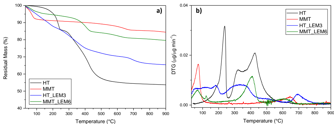
Figure 5. (a) TG (a) and DTG (b) results obtained for HT, MMT and lemon hybrid pigments (HT-LEM and MMT-LEM).
