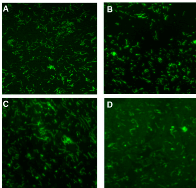
FIGURE 1. Indirect immunofluorescence assay detection of Borrelia crocidurae Achema strain ( A and B ; magnification: \times 400 ) and clinical isolate B. crocidurae 03-02 ( C and D ; magnification: \times 600 ) by purified mouse monoclonal antibodies (MAbs): P3A10 ( A and C at 1:500 and 1:1,000 dilution, respectively) and P6D9 ( B and D at 1:500 and 1:1,000 dilution, respectively). Monoclonal antibodies were tagged using a goat anti-mouse IgG conjugated to fluorescein isothiocyanate at 1:400 dilution. These two mentioned MAbs are available for research purposes upon request from the corresponding author.
