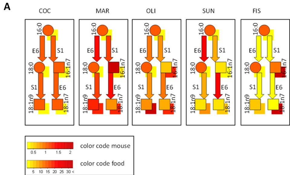
Fig. 4 a Metabolic pathways of SCD1 (S1) and ELOVL6 (E6) mediation of 16:0 and 18:0–16:1n7, 18:1n7 and 18:1n9 in plasma phospholipids and dietary fats effects. The supplemented dietary fat is shown as a shadow behind the individual fatty acid in plasma phospholipids. b Proposed mechanisms for fish oil supplementation and modification of hepatic CYP26A1 expression and concomitant effects on SAFA to MUFA synthesis via SCD1 and ELOVL6 expression. COC coconut fat, MAR margarine, OLI olive oil, SUN sunflower oil, FIS fish oil
