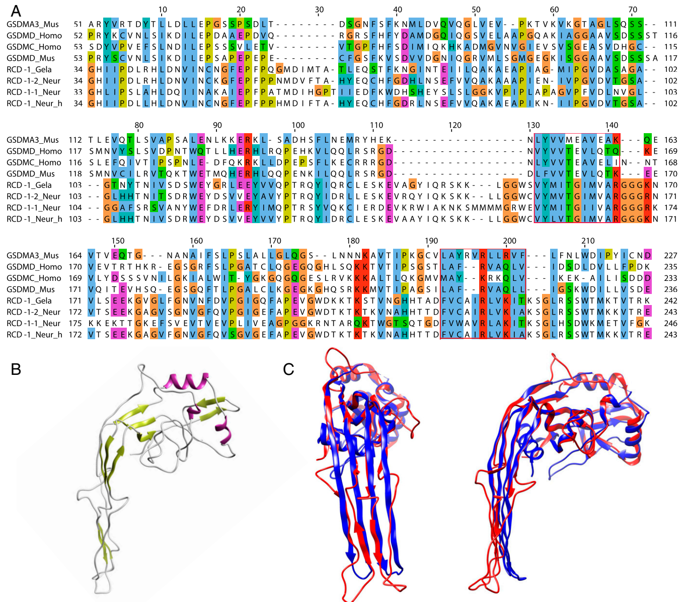
Fig. 1. Protein alignment and molecular models of the pore-forming N-terminal domains of mammalian gasdermins and fungal RCD-1 proteins. (A) Alignment of protein sequences of murine (Mus) gasdermin-A3 (NP_001007462), gasdermin-D (NP_081236), human (Homo) gasdermin-D (NP_079012), gasdermin-C (NP_113603) with RCD-1-1 (XP_962898) and RCD-1-2 from N. crassa (Neur) and RCD-1 variants from N. hispaniola (Neur_h) and Gelasinospora tetrasperma . Conserved residues are shown in ClustalX colors, based on the nature of the amino acid residues: hydrophobic – blue, polar – green, negative charge – magenta, positive charge – red, aromatic – cyan, glycine – orange, proline – yellow, cysteine – pink, any/gap – white. Two highly conserved blocks between all sequences are boxed in red. (B) Template-based model of the RCD-1-2 allelic variant from Neurospora crassa . Murine GSDMA3 (6CB8) in the active pore-forming state was determined ( P value = 7.22e-05 ) as the best template based on the sequence input (RCD-1-2). (C) Structural alignment of GSDMA3 (6CB8A) (blue) and the generated model of RCD-1-2 (red). Shown are a frontal view (Left) and side view (Right) of the two overlaid structures.
