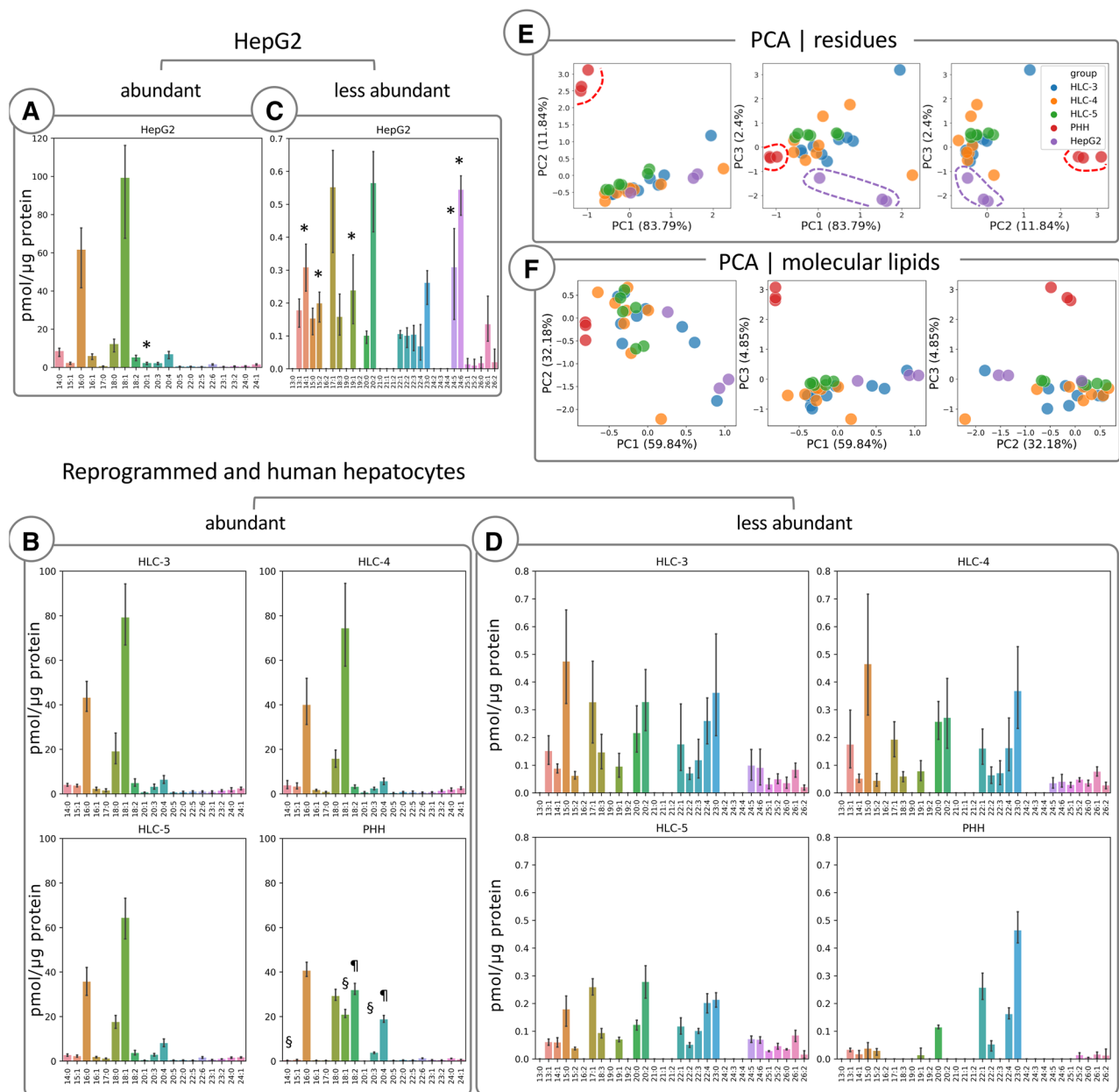
Figure 1. Lipidomics data from cultured primary hepatocytes, reprogrammed hepatocytes and HepG2 cells is reprocessed with liputil. Residues extracted from lipidomic data of HepG2, human hepatocyte-like cells (HLCs) and human primary hepatocytes (HPPs) are shown (A–D, n=9 HLC-3, n=8 HLC-4, n=6 HLC-5, n=3 PHH and HepG2 samples). Units were unchanged during the extraction and are the same as the input data (pmol/ \mu g protein). * p < 0.05 vs PHH, HLC-3, HLC-4 and HLC-5; § p < 0.01 vs HepG2, HLC-3 and HLC-4; ¶ p < 0.0001 vs HepG2, HLC-3, HLC-4 and HLC5. * indicates the similarities between PHHs and HLCs vs HepG2; ¶ and § indicate the similarities between HepG2 and HLCs vs PHHs. Statistically significant differences were determined with ANOVA followed by Tukey’s post-hoc test. Detailed statistics can be found in Supplementary Table S1. Histograms show the average \pm SD. Scatter plots of the first three principal components (PCs) are shown for residues of each sample (E) and for molecular lipids for each sample (F).
