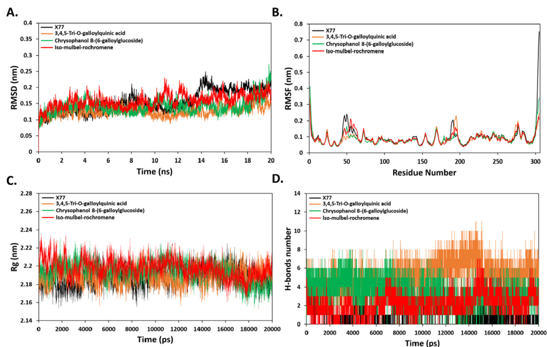
Fig. 5 (A) RMSD of backbone atoms (C, C \alpha , and N) for 3CL PRO -Ligand complex systems. (B) RMSF of backbone atoms for 3CL PRO -Ligand complex systems. (C) Radius of gyration (Rg) of backbone atoms (D) Number of H-bonds over 20 ns simulation time.
