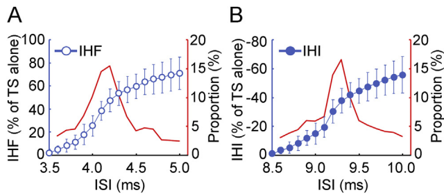
Fig. 3. Latency distribution measurement. Latency distribution of transcallosal fibers measured with (A) IHF and (B) IHI in one subject. The ISI range from no IHF (or IHI) to the maximal IHF (or IHI) was shown. Abscissa indicates the ISI. Left ordinate (blue) in each panel indicates the magnitude of IHF (blue open circle) or IHI (blue filled circle). It is expressed as a percentage difference between motor evoked potential amplitude induced by CS-TS paired-pulse stimulation and that induced by TS alone (defined as 100%). The value for IHF is positive and that for IHI is negative. Right ordinate (red) in each panel indicates the proportion of the nerve fibers with certain conduction velocity in the whole bundle. The proportion for a group of nerve fibers (red curve) was represented by the percentage of the difference in IHF (or IHI) with the minimal increase in ISI (0.1 ms) divided by the maximal IHF (or IHI). The curve was smoothed with a two-point moving average. Note that the peak proportion of transcallosal fibers measured with IHF and that with IHI were similar. CS = conditioning stimulus, IHF = interhemispheric facilitation, IHI = interhemispheric inhibition, ISI = interstimulus interval, TS = test stimulus. (For interpretation of the references to color in this figure legend, the reader is referred to the Web version of this article.)
