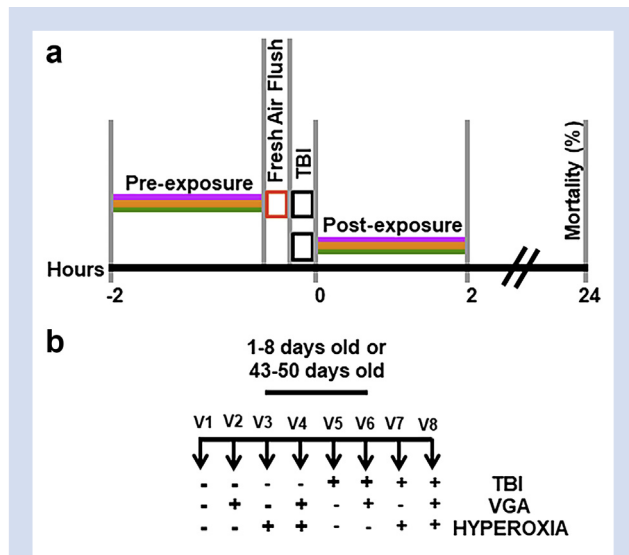
Fig 2. Diagram of the workflow for experiments presented in Figs 2 and 3 . (a) Timelines for Pre-exposure vs. Post-exposure to anaesthetics and hyperoxia relative to traumatic brain injury (TBI). The standard exposure duration was 2 h of 2% isoflurane (ISO), 3.5% sevoflurane (SEVO), and/or 100% O 2 (purple, yellow, and green lines, respectively). After pre-exposure, the anaesthetic was flushed for 5 min (red rectangle). TBI was administered with 5 min intervals between strikes. (b) Experimental schematic illustrating all of the experimental and control conditions. Vials one through eight (V1eV8) were considered one experimental unit. Horizontal rows show exposure to interventions (b) or lack thereof (e). For example, V1 undergoes no intervention and serves as control for natural attrition. V5 undergoes only TBI. See methods and statistical appendix in supplementary material for details.
