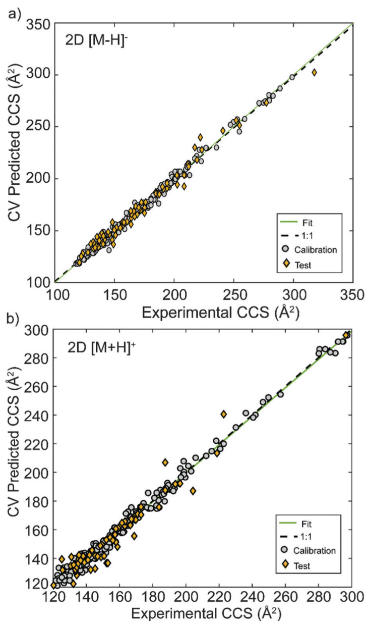
Fig. 1. Measured vs. cross-validation (CV)-predicted CCS for metabolites developed using (a) 2D structural files to calculate molecular descriptors for [M - H]^- adducts, and (b) 2D structural files to calculate molecular descriptors for [M + H]^+ adducts. Optimal molecular descriptors were selected by a genetic algorithm.
