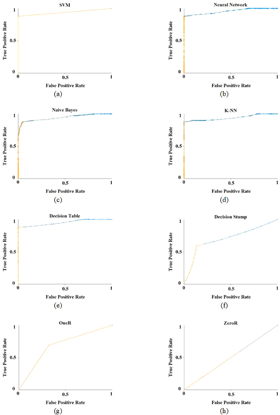
Fig. 4. ROC curves. (a) SVM. (b) Neural Network. (c) Naive Bayes. (d) K-NN. (e) Decision Table. (f) Decision Stump. (g) OneR. (h) ZeroR.
