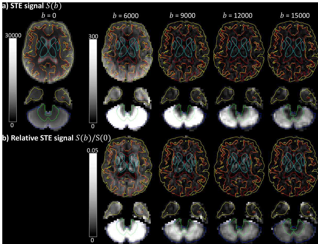
Fig. 3. a) STE signal as a function of b-value (in \text{s/mm}^2 ), with the Freesurfer tissue segmentations indicated in red = WM, yellow = GM, cyan = deep GM, green = cerebellar WM and blue = cerebellar GM. b) Relative STE signal change.
