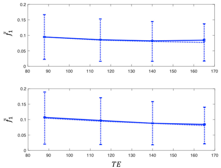
Fig. 7. a) Parameter estimates \tilde{T}_2 and \tilde{D}_1 , in the cGM ROI. D has units \mu\text{m}^2/\text{ms} and T2 has units ms. b) Parameter estimates \hat{f}_1 in the cGM ROI (median and 10–90 percentile) as a function of TE. The dotted errorbars represent the median and 10–90 percentile, and the solid (very narrow) errorbars the mean and standard error of the mean. TE has units ms.
