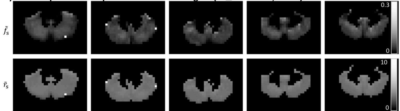
Fig. 8. a) Left: STE signal simulation of a spherical compartment for different values of D_s and r_s , r_s is given in \mu\text{m} . Right: estimates of D_1 in \mu\text{m}^2/\text{ms} (Eq. [3]) for different values of D_s and r_s . b) Estimates of f_s and r_s in the cerebellar GM of five healthy controls, assuming D_s = 3 \mu\text{m}^2/\text{ms} .
