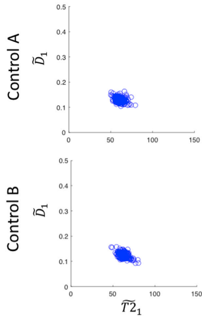
Fig. 7. a) Parameter estimates \tilde{T}_2 and \tilde{D}_1 , in the cGM ROI. D has units \mu\text{m}^2/\text{ms} and T2 has units ms. b) Parameter estimates \hat{f}_1 in the cGM ROI (median and 10–90 percentile) as a function of TE. The dotted errorbars represent the median and 10–90 percentile, and the solid (very narrow) errorbars the mean and standard error of the mean. TE has units ms.
