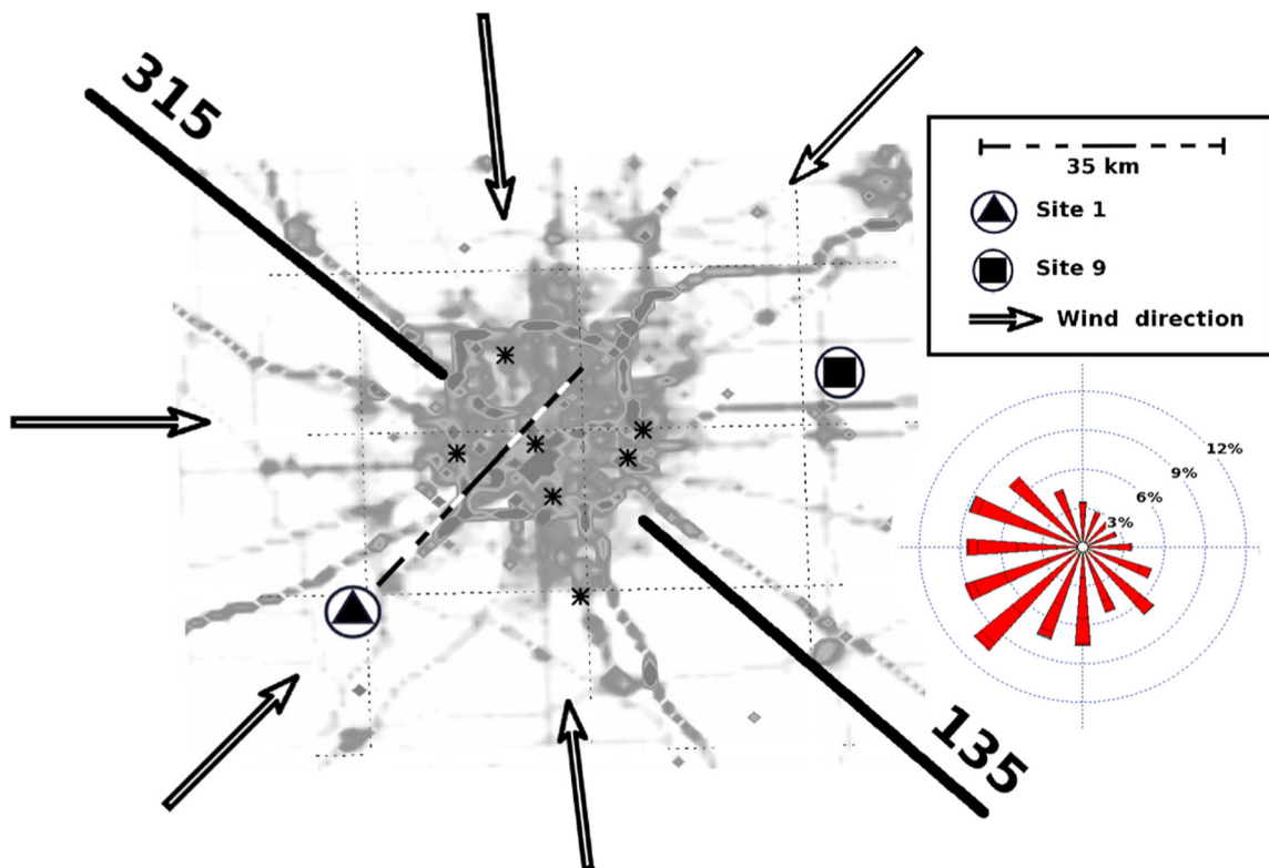
Figure 4. Selection of the background site to determine the upwind concentrations of CO 2 over Indianapolis, using two semicircles (135° and 315°) and hourly modeled wind directions from the WRF-FDDA system at three locations across the city. The emitting area defined by Hestia is represented in gray. The distance between Site 1 and Site 9 (about 35 km) corresponds to an advection time of about 2 h. The wind climatology for the month of December at the Indianapolis airport (IND station) is shown under the legend (in red).
