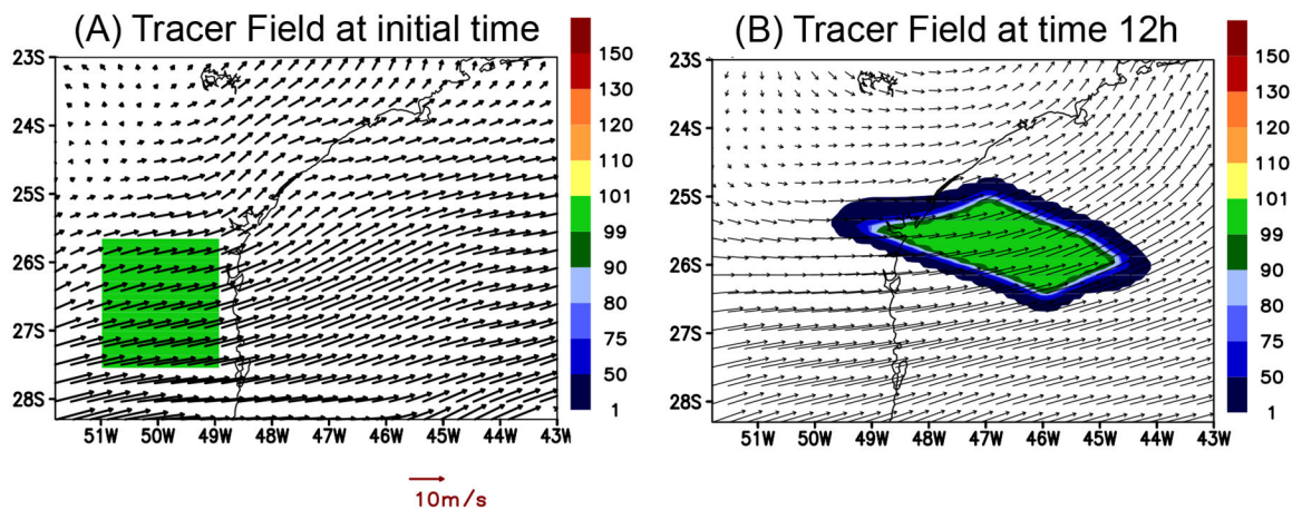
Figure 1. A 3-D hypothetical case study: transport of a rectangular parallelepiped by a realistic divergent flow over the Southeast part of Brazil. (A) The tracer concentration field expressed in terms of mass mixing ratio at initial time and 1900 m height; the horizontal wind flow is also depicted. (B) The correspondent mass mixing ratio after 12 hours as simulated by the monotonic advection scheme.
