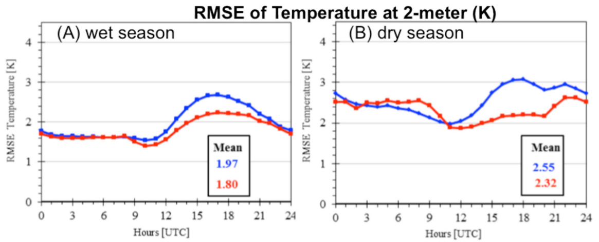
Figure 4. RMSE of air temperature at 2 meters using JULES (in red) and LEAF3 (in blue) surface schemes with BRAMS over South America during (A) wet season in March 2010, and (B) dry season in September 2010.
