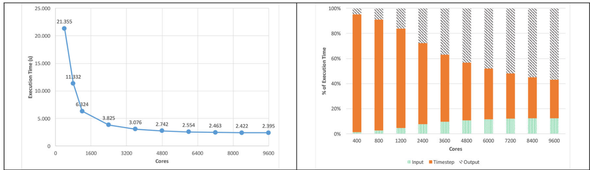
Figure 21. Execution time at TUPA of the 5 km grid and processes responsibility
