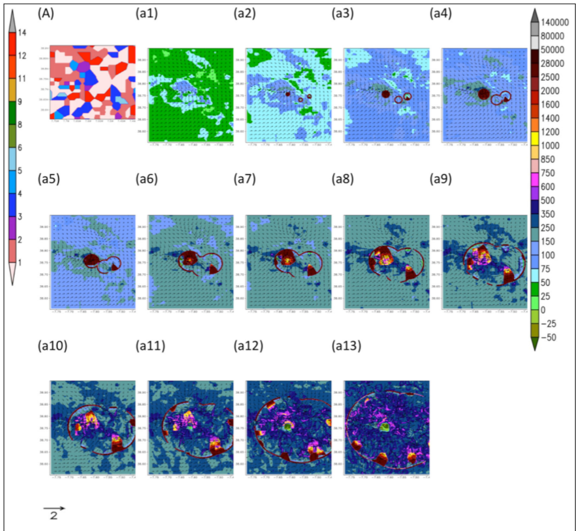
Figure 23. (A) Fuel models of Ossa mountain range region. Panels from a1 to a13 show sensible heat fluxes ( Wm^{-2} ) during the fireline spread and behavior of horizontal atmospheric wind ( ms^{-1} ) influence of the fire in different moments of forestry fire occurred in 7/8/2006 in Ossa mountain range in Alentejo in Portugal, simulated by BRAMS-SFIRE.
