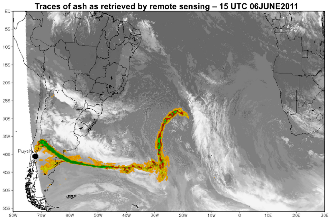
Figure 16. Traces of volcanic ash associated with eruption of the Puyehue volcano as retrieved from METEOSAT-8 satellite data. The image corresponds to 15UTC 06 June 2011.
