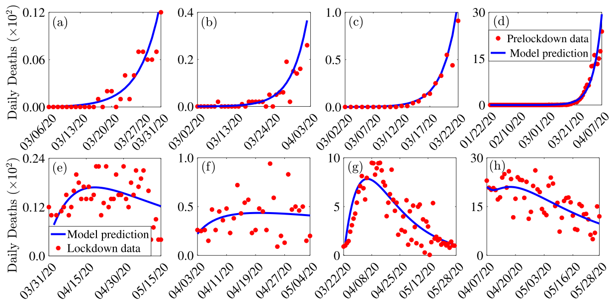
Fig. 3. Simulations of the model (2.1) using values of the 13 known parameters of the model obtained from the literature (given in Table A3 in Appendix A) and those for the 12 unknown parameters obtained from fitting the model with the cumulative COVID-19 mortality data (given in Tables A4–A7 in Appendix A). (a)–(d): Daily mortality data and daily mortality prediction generated from the model for the pre-lockdown period for the states of Arizona, Florida, New York, and for the entire US, respectively. (e)–(h): Daily mortality data and daily mortality prediction from the model for the lockdown period for the state of Arizona, Florida, New York and the entire US, respectively. The data is displayed in red dots.
