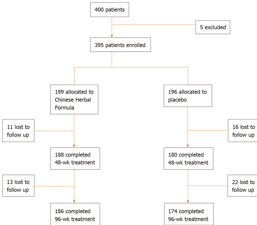
Figure 1 Study flowchart.
