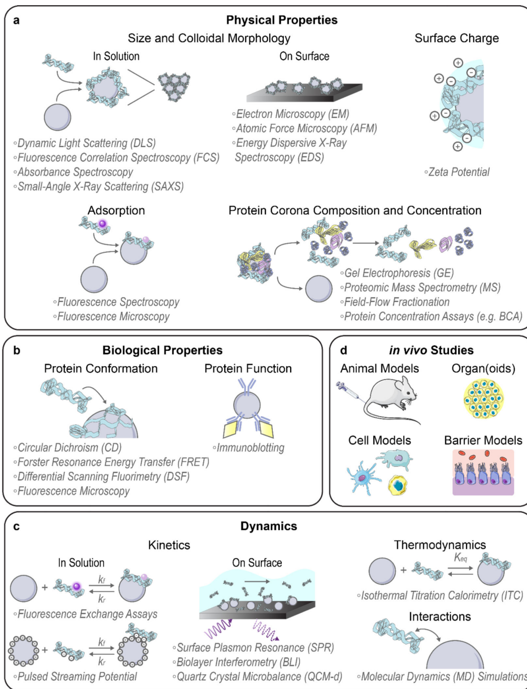
Figure 2. Modes of characterizing protein-nanoparticle complex formation and performance. (a) Physical properties include complex size and colloidal morphology (preferably characterized in solution over on surface), surface charge, corona adsorption, and corona composition and amount. (b) Biological properties include surface-adsorbed protein conformation and function. (c) Dynamics include kinetics (preferably characterized in solution over on surface), thermodynamics, and interactions. (d) in vivo function can be assessed in model organisms, organs or organoids, cells, and cellular barriers. Some images
