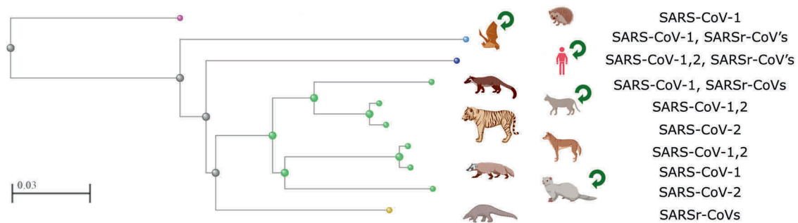
Fig. 3 Phylogeny of observed wild infections. Left panel, fast minimum evolution distance tree for ACE2 protein sequences using Grishin for evolutionary distance, unsorted. Species included are Erinaceus europaeus (in place of Erinaceus amurensis , Hedgehog), Rhinolophus sinicus (representative microbat), Nyctereutes procyonoides (Raccoon Dog), Manis javanica (Sunda Pangolin), Paguma larvata (Masked Palm Civet), Mustela putorius furo (representative ferret), Panthera tigris altaica (Siberian Tiger, in place of Bengal Tiger), Canis lupus familiaris (Dog), Neovison vison (in place of European Mink). The closest species was used where applicable due to a lack of sequence for ACE2. Right side indicates whether infection was observed for SARS-CoV, SARS-CoV-2 or SARSr-CoV (Bat SARS-Like CoV's), as indicated. Green arrows indicate where animal-animal transmission has been reported to occur.
