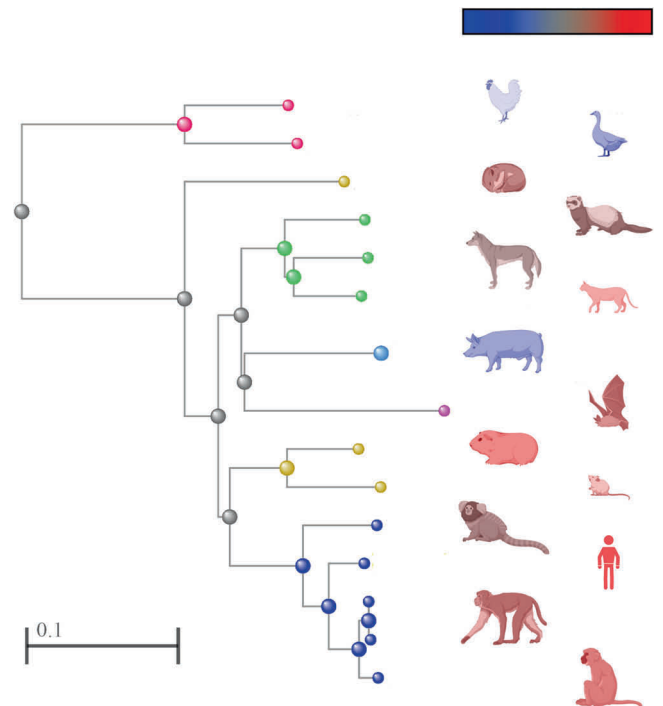
Fig. 1 ACE2 protein phylogenetic divergence and in vivo model severity. Left panel, fast minimum evolution distance tree for ACE2 protein sequences using Griphin for evolutionary distance, unsorted. Species included are Gallus gallus (Chicken), Anas platyrhynchos (Duck), Cavia porcellus (Guinea Pig), Mustela putorius furo (Ferret), Canis lupus familiaris (Dog), Felis catus (Cat), Sus scrofa (Pig), Roussettus aegyptiacus (fruitbat), Mesocricetus auratus (Golden hamster), Mus musculus (Mouse), Callithrix jacchus (Common Marmoset), Macaca mulatta (Rhesus macaque), Macaca fascicularis (Cynomolgus Macaque), Chlorocebus aethiops (African Green Monkey) and Homo sapiens . Macaques are represented as one image due to close divergence. Severity of disease is color-coded from refractory to infection (BLUE, no virus detected) to severe (RED, shedding). Common Marmoset and Guinea Pig have only been assessed for SARS-CoV, all others with SARS-CoV-2. Scale indicates 10% amino acid divergence.
