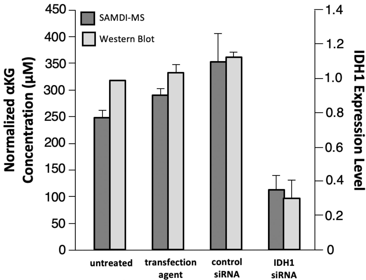
Fig. 6. IDH1 expression level as determined with western blot and αKG concentration as measured with SAMDI-MS for untreated cells and cells treated with transfection agent, control sequence siRNA and IDH1-targeting siRNA. All data are expressed as mean ± standard deviation with n = 2 experimental replicates.
