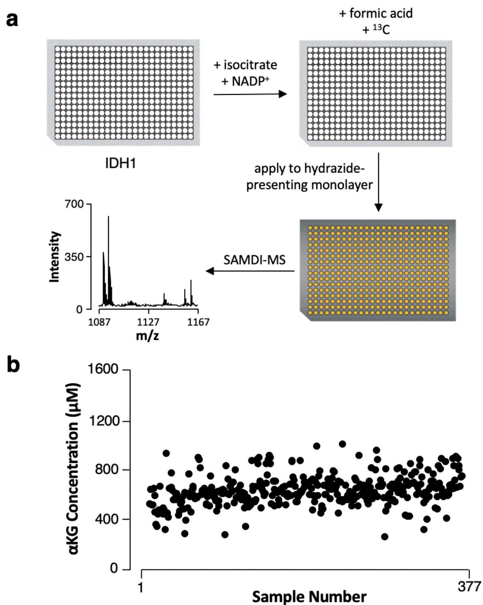
Fig. 4. (a) Scheme for the preparation and analysis of recombinant IDH1 samples. (b) \alpha KG concentrations measured in the 384-sample biochemical screen (7 samples did not produce either ^{12}\text{C} or ^{13}\text{C} \alpha KG capture).
