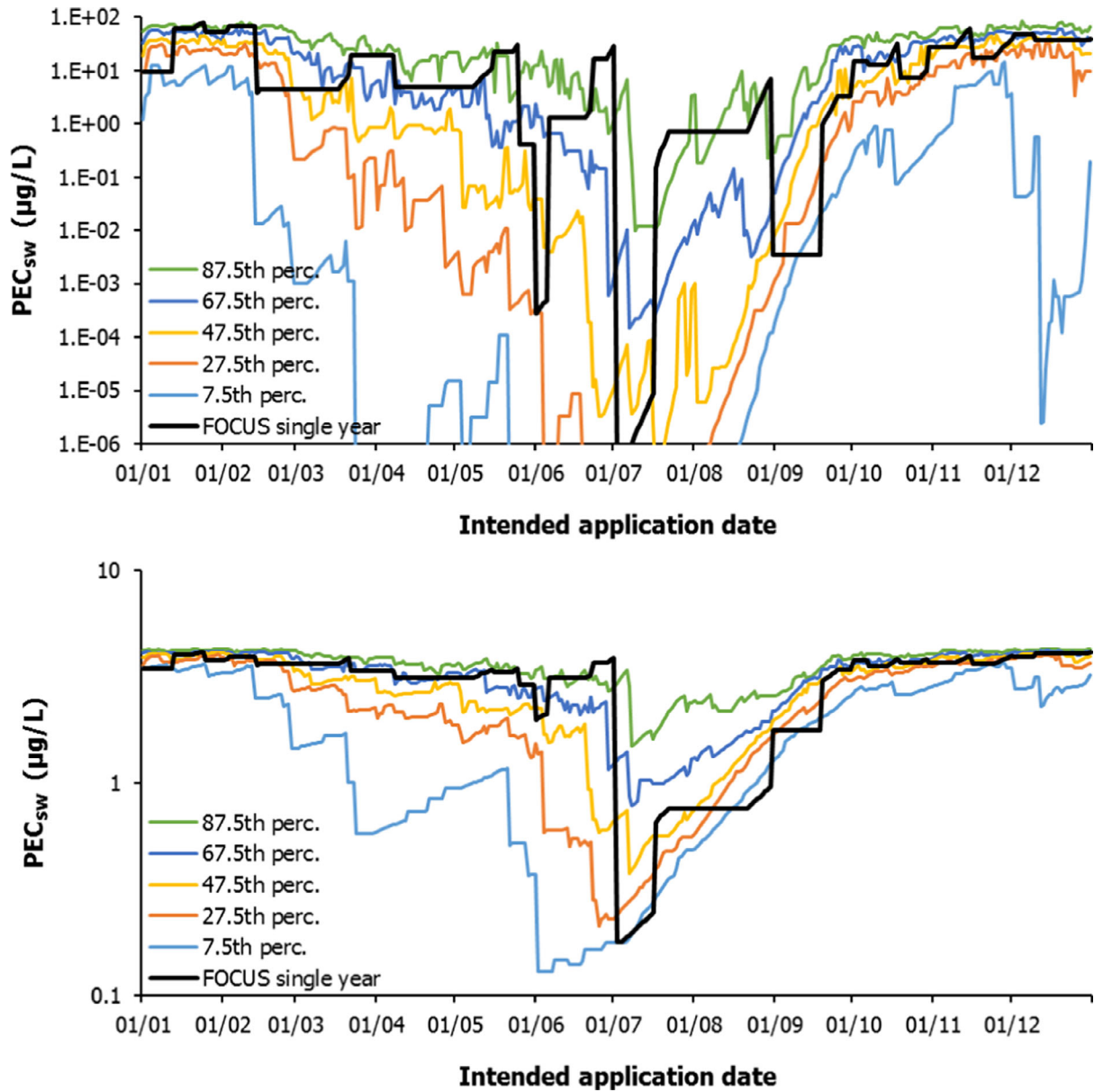
Figure I.10: PEC_{sw} ( \mu\text{g/L} ) for dummy substance A (top) and dummy substance F (bottom) in the run-off scenario R2 based on the new 20-year assessment approach (7.5th to the 87.5th percentile, 7-day application window) and the current FOCUS single-year assessment approach, in relation to the intended application date (potatoes, 1 \times 1 \text{ kg/ha} to the soil surface, no drift). Data are based on a TOXSWA stream meta model
