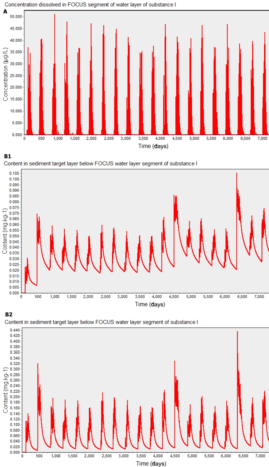
Figure A.4: R4-Roujan, stream simulated with dummy substance I; six applications of 1 kg/ha in maize. (A) Concentration in water layer (µg/L), (B1) Content in upper 5 cm of sediment, (B2) Content in upper 1 cm of sediment (both in mg/kg dry sediment)
