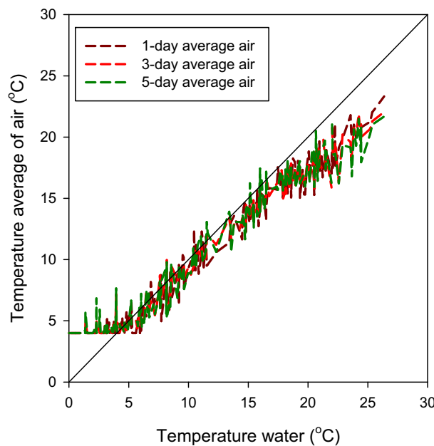
Figure P.5: Measured average daily water temperatures and 1-day, 3-day and 5-day averaged air temperatures for the Zeeland pond in August 2008
